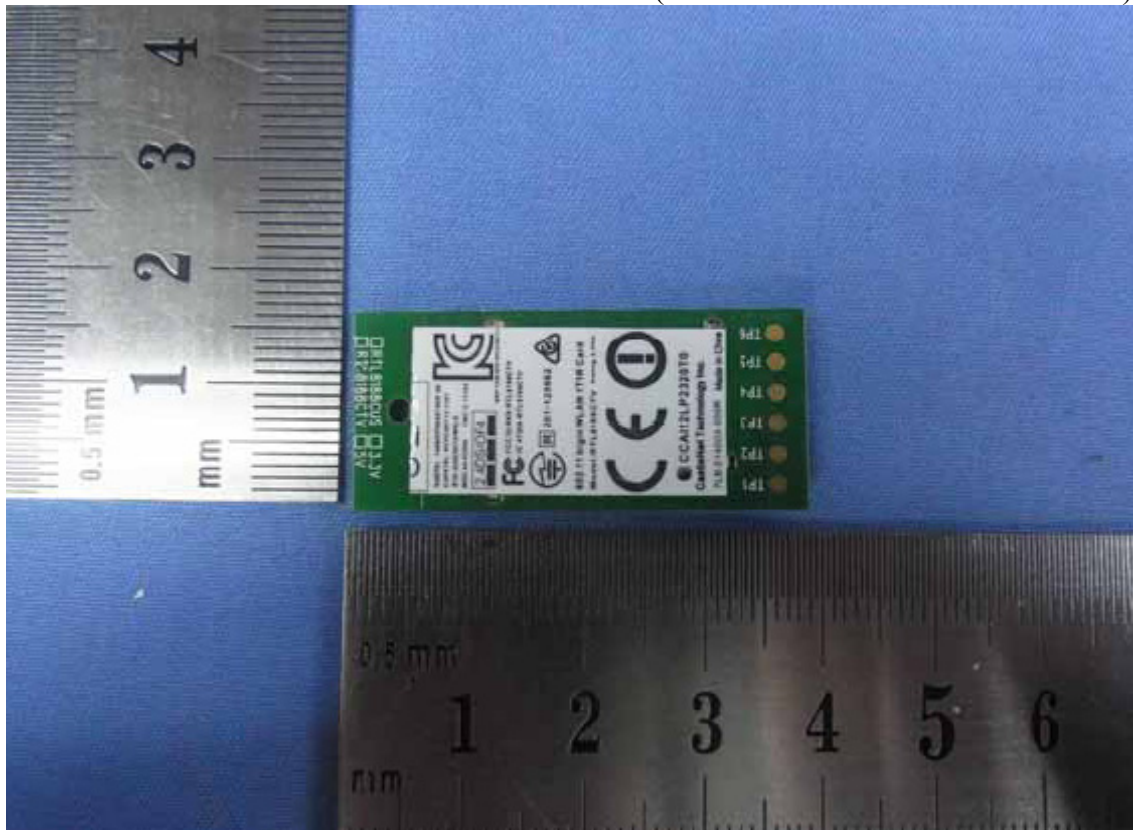
Figure 17 Internal View (WLAN Module Board / Back View)
