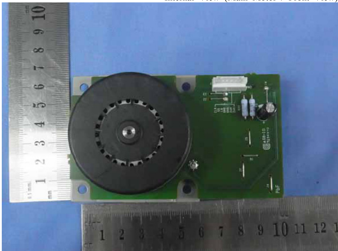
Figure 18 Internal View (Main Motor / Front View)
