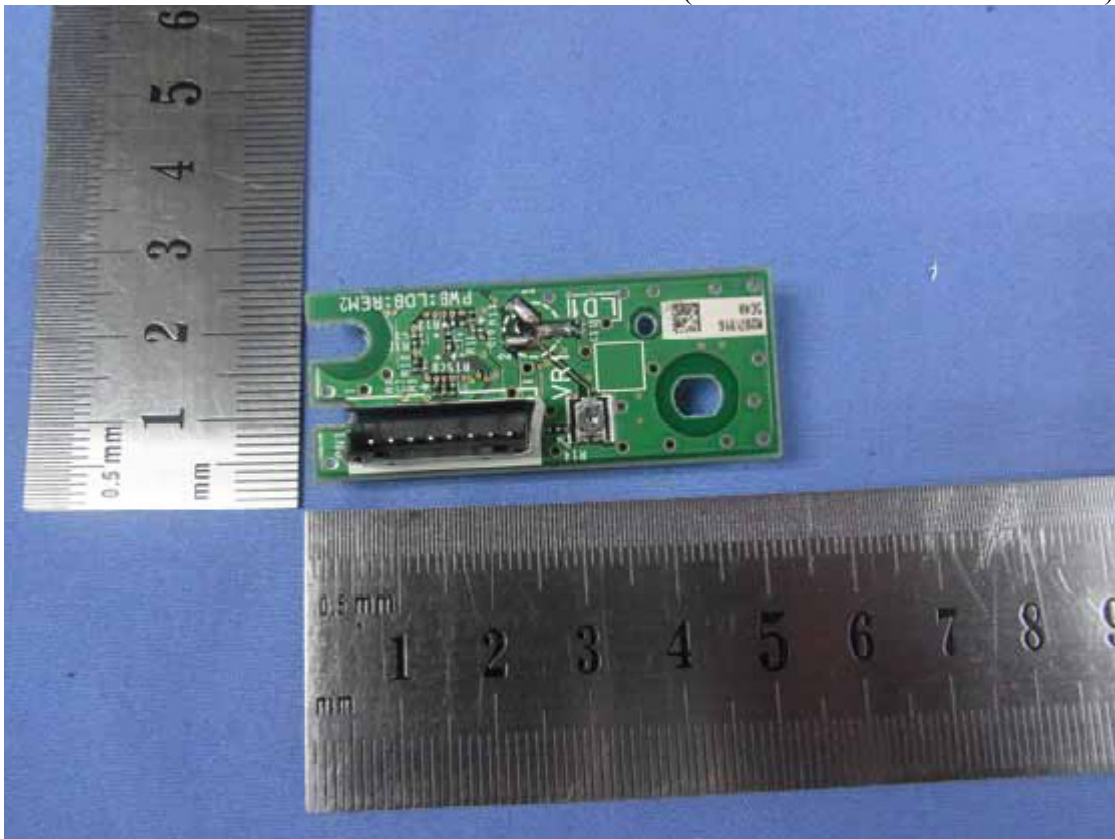
Figure 16 Internal View (WLAN Module Board / Front View)
