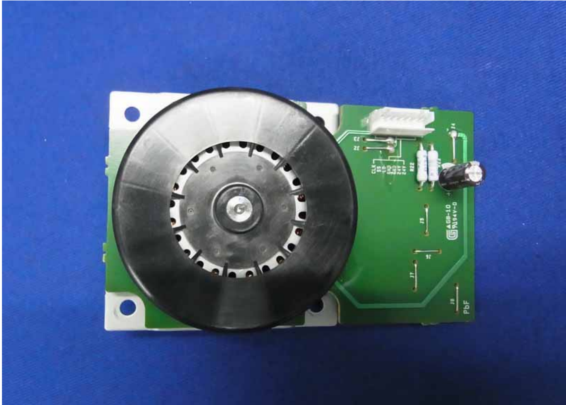
Figure 19 Backside of the PCB
