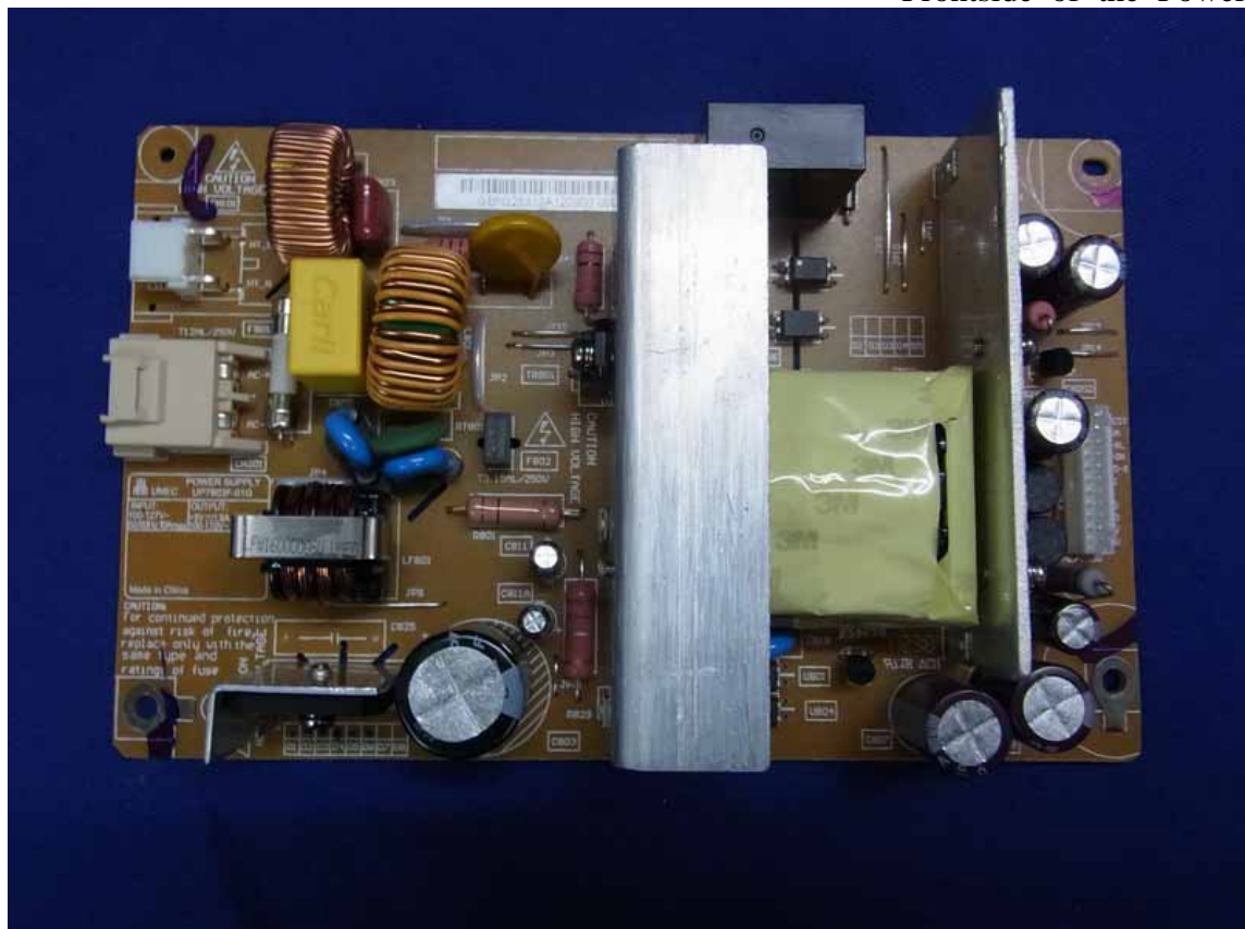
Figure 12 Frontside of the Power Board
