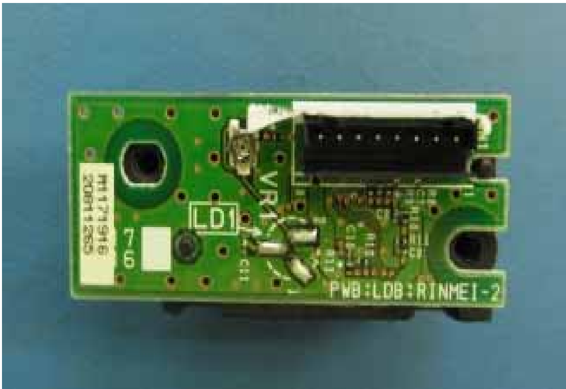
Figure 14 Frontside of the PCB
