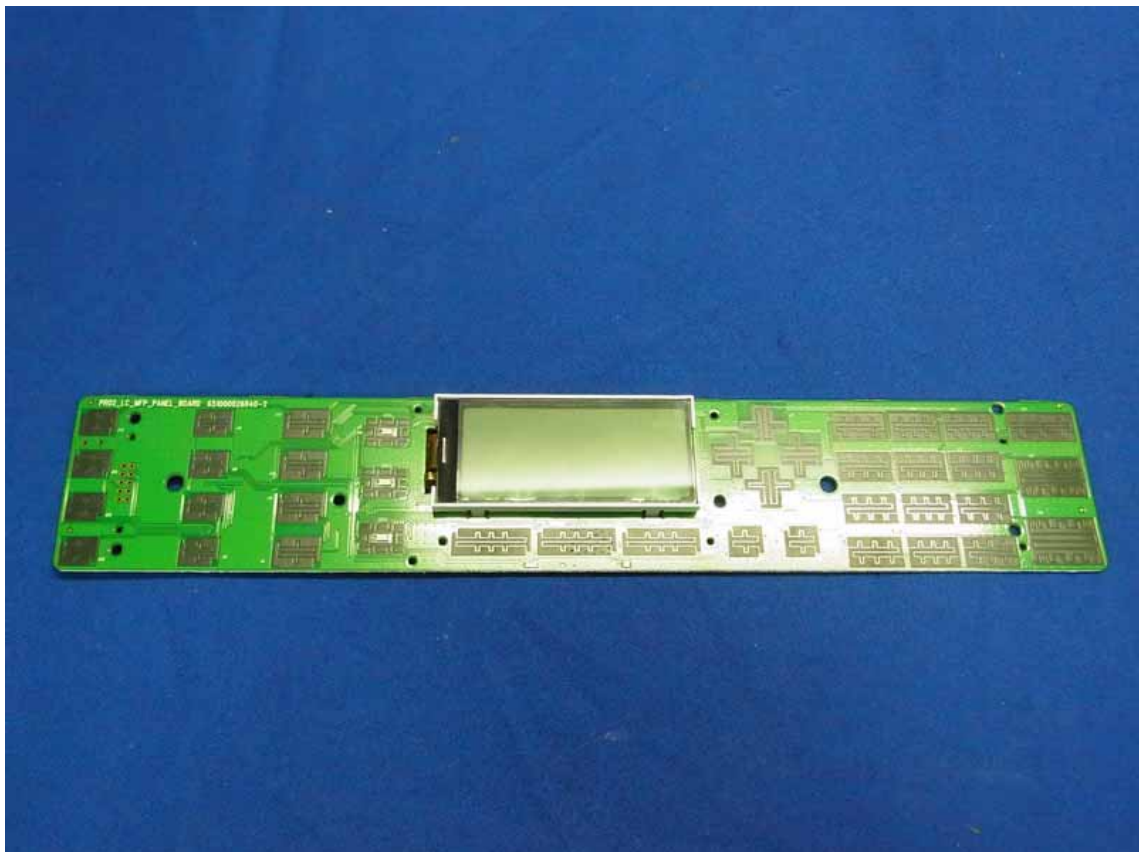
Figure 28 Frontside of the PCB
