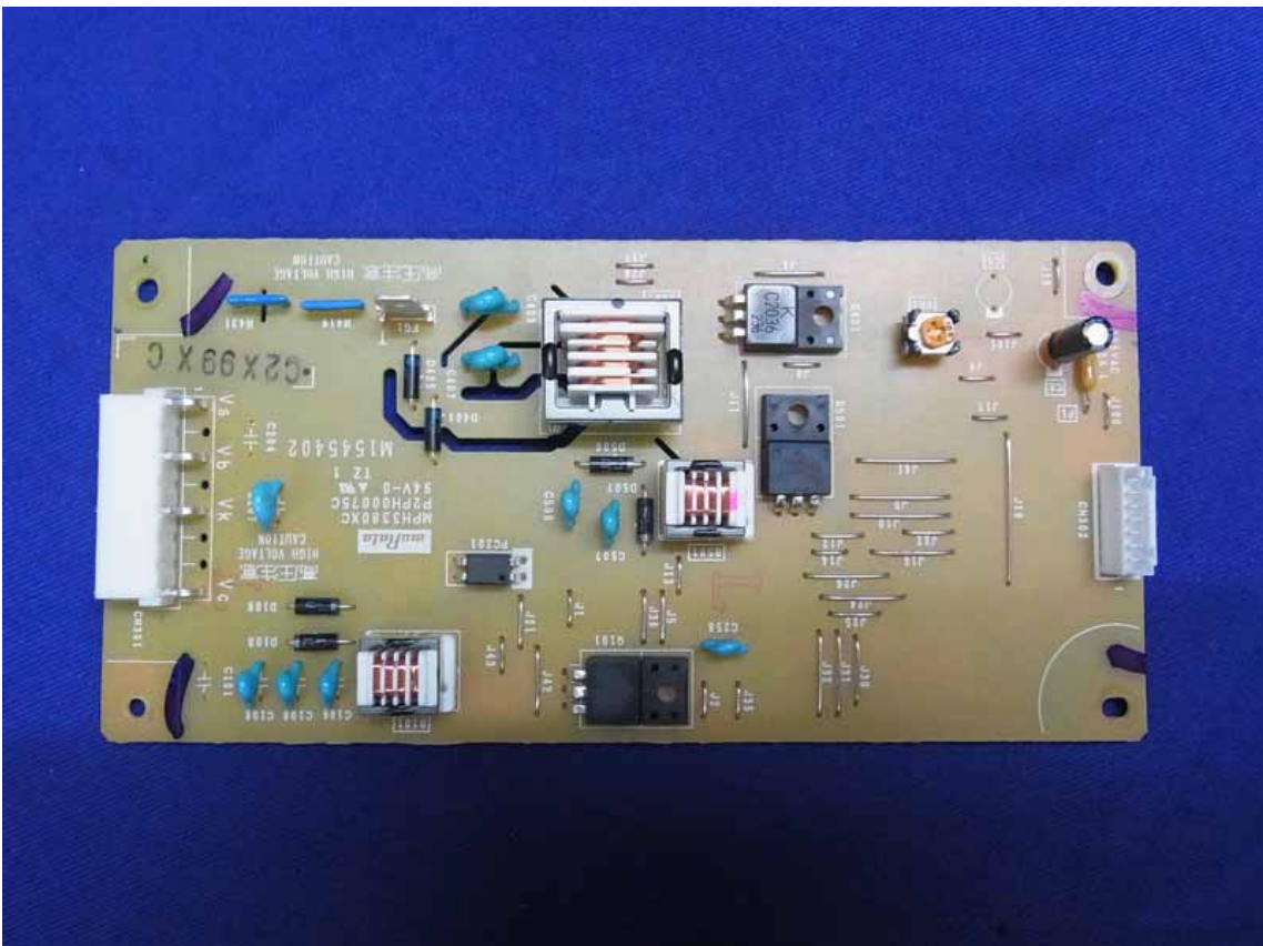
Figure 16 Frontside of the PCB
