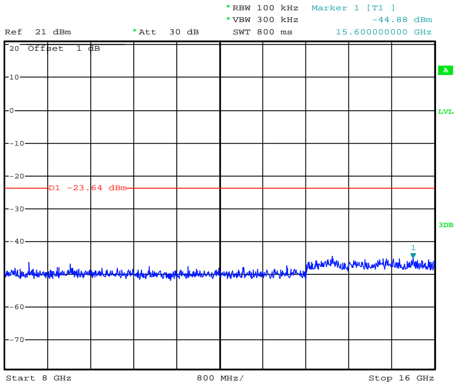
(Plot 4.6.4 A2: Channel 3: 2422MHz @ 802.11n(40MHz))
