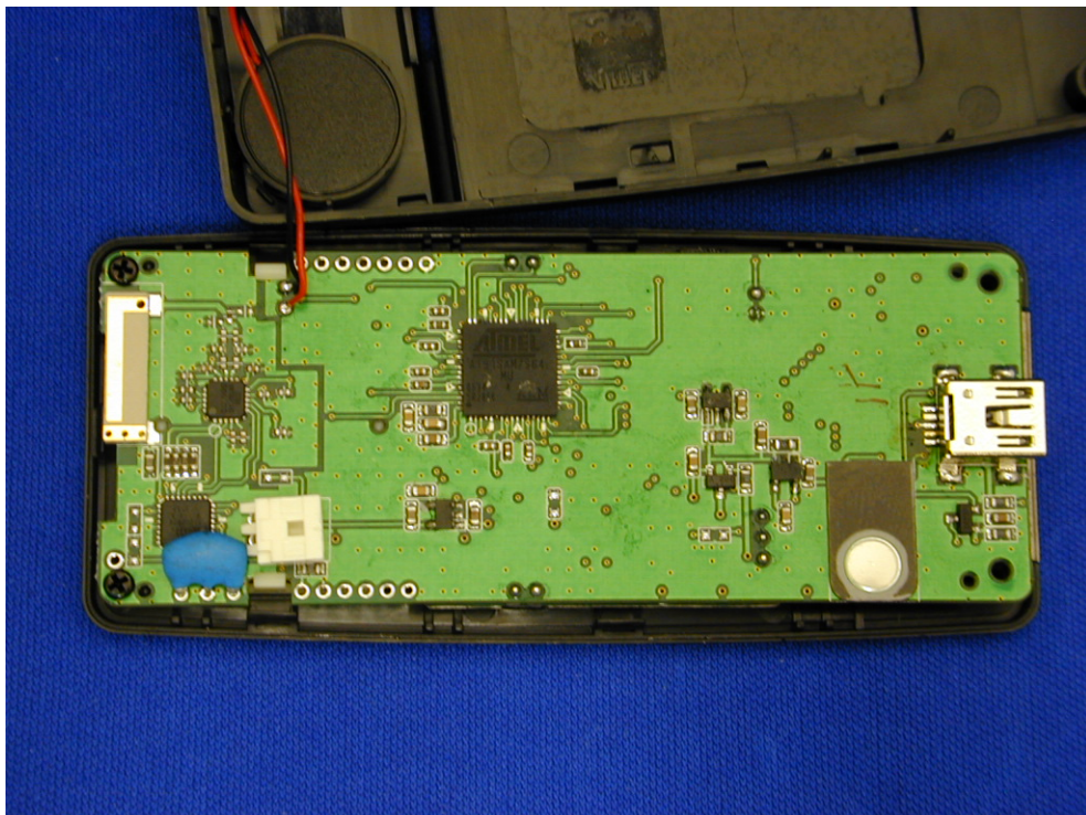
PCB Back
