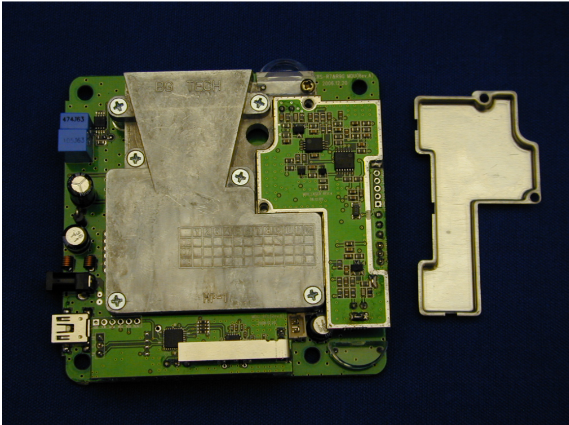
PCB Top w/o Shield
