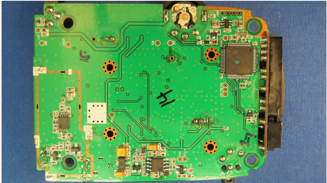
Bottom View laser shield removed
