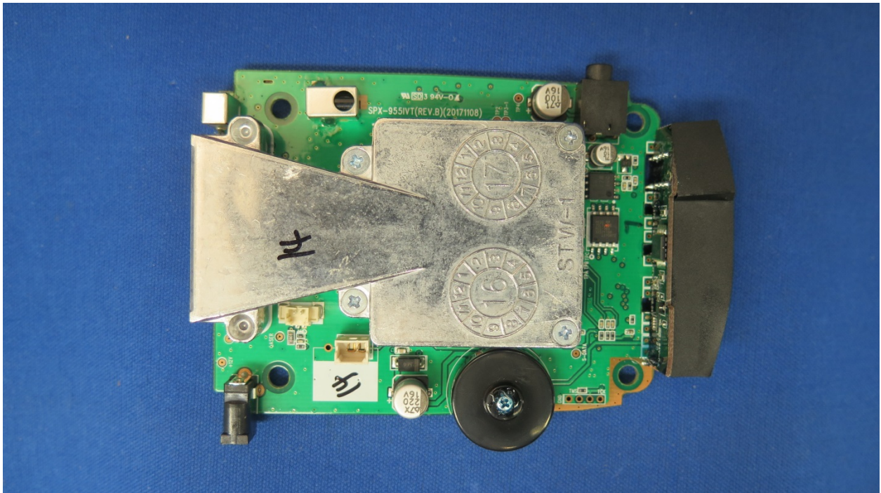
Top View PCB Top Horn Removed
