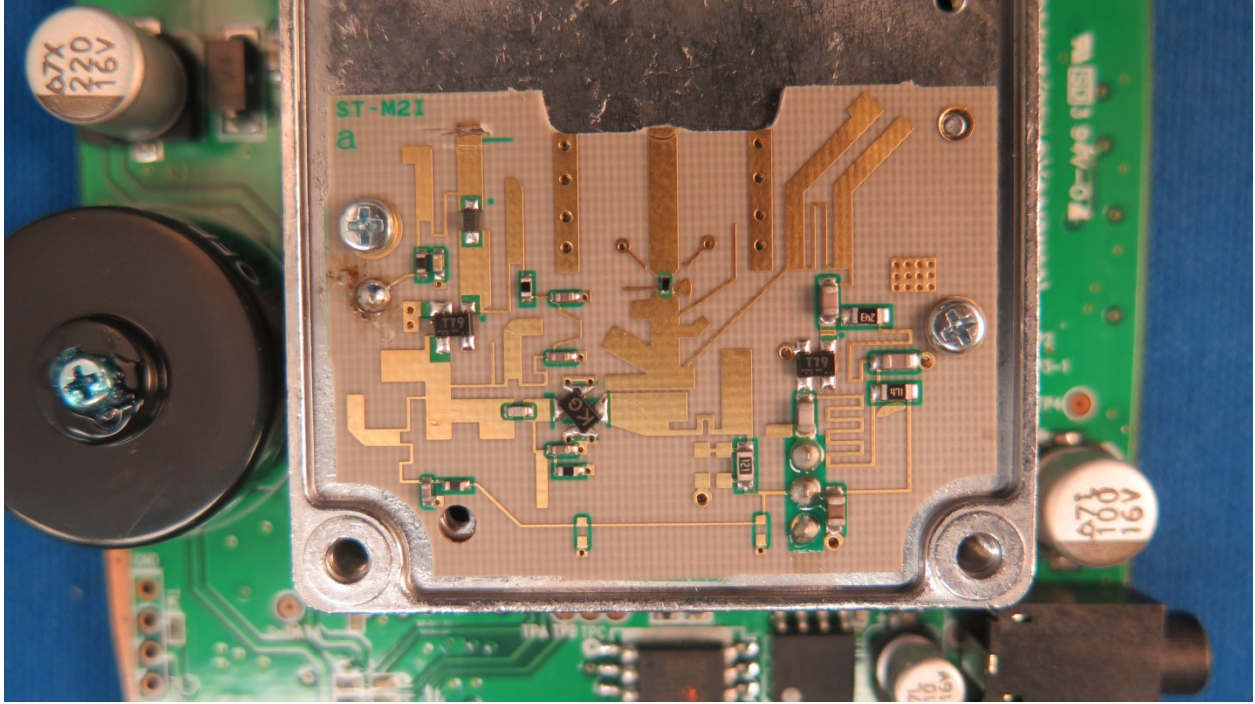
Close Up – LNA PCB
