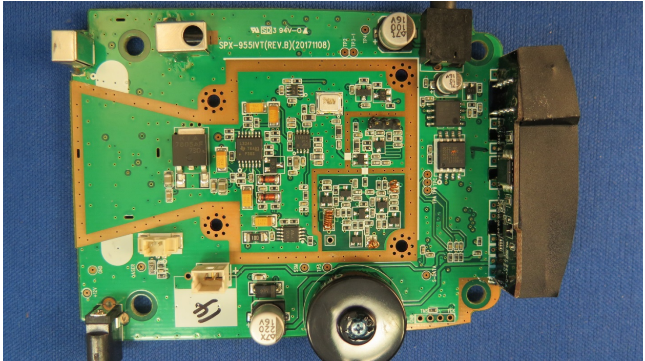
Top View – PCB Horn Removed
