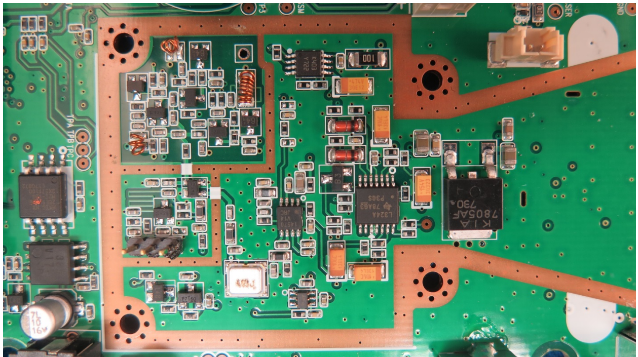
Top View – PCB Horn Removed – B
