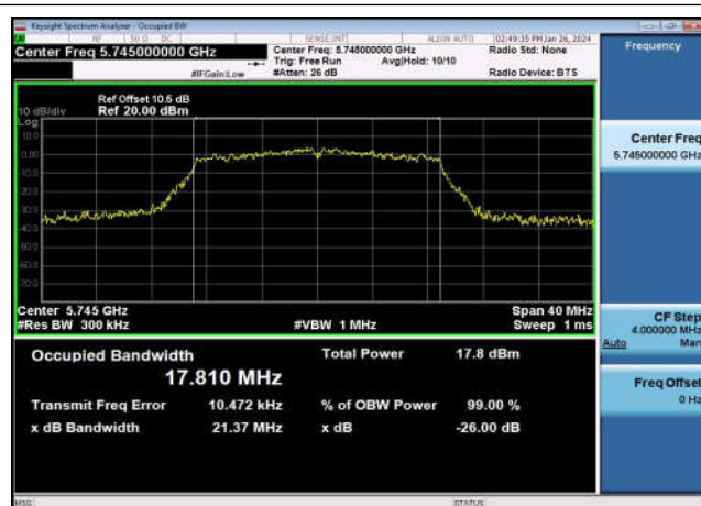
U-NII-3 99% & 26dB Bandwidth-802.11ac(20MHz) ,5745MHz,Ant1
