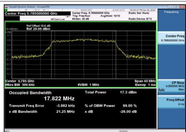
U-NII-3 99% & 26dB Bandwidth-802.11ac(20MHz) ,5785MHz,Ant1
