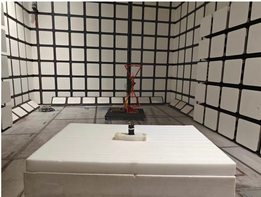
Radiated Emissions View (Below 1 GHz) – Model: Performa 400
