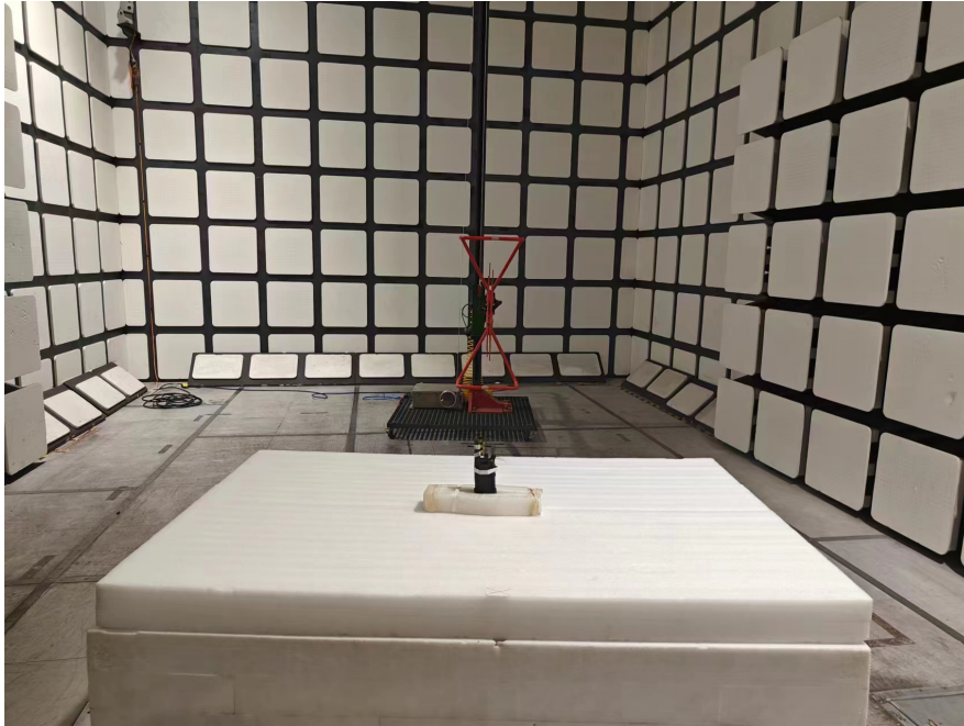
Radiated Emissions View (Below 1 GHz) – Model: Performa 450
