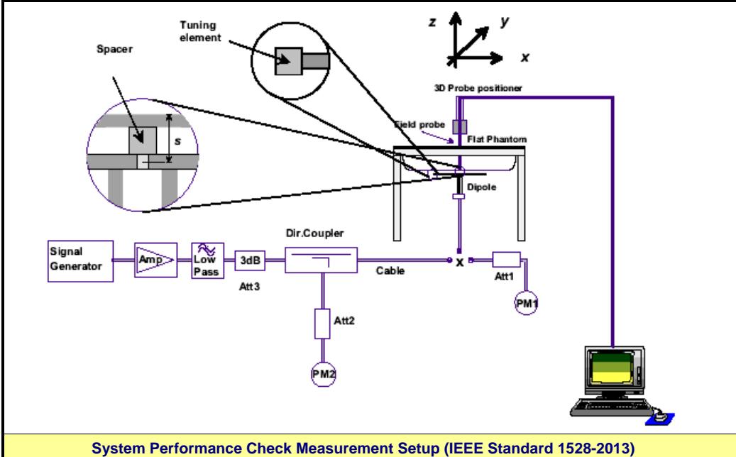
SPEAG 300 MHz Validation Dipole Setup
