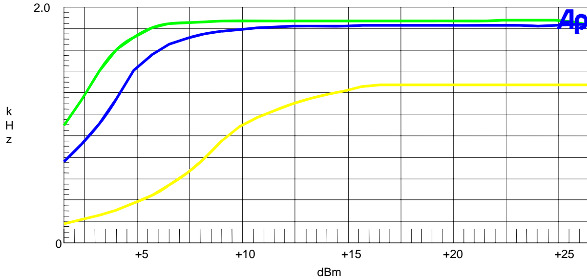
MODULATION LIMITING PLOT GREEN 2.5kHz -- BLUE 1.0kHz -- YELLOW 300Hz
