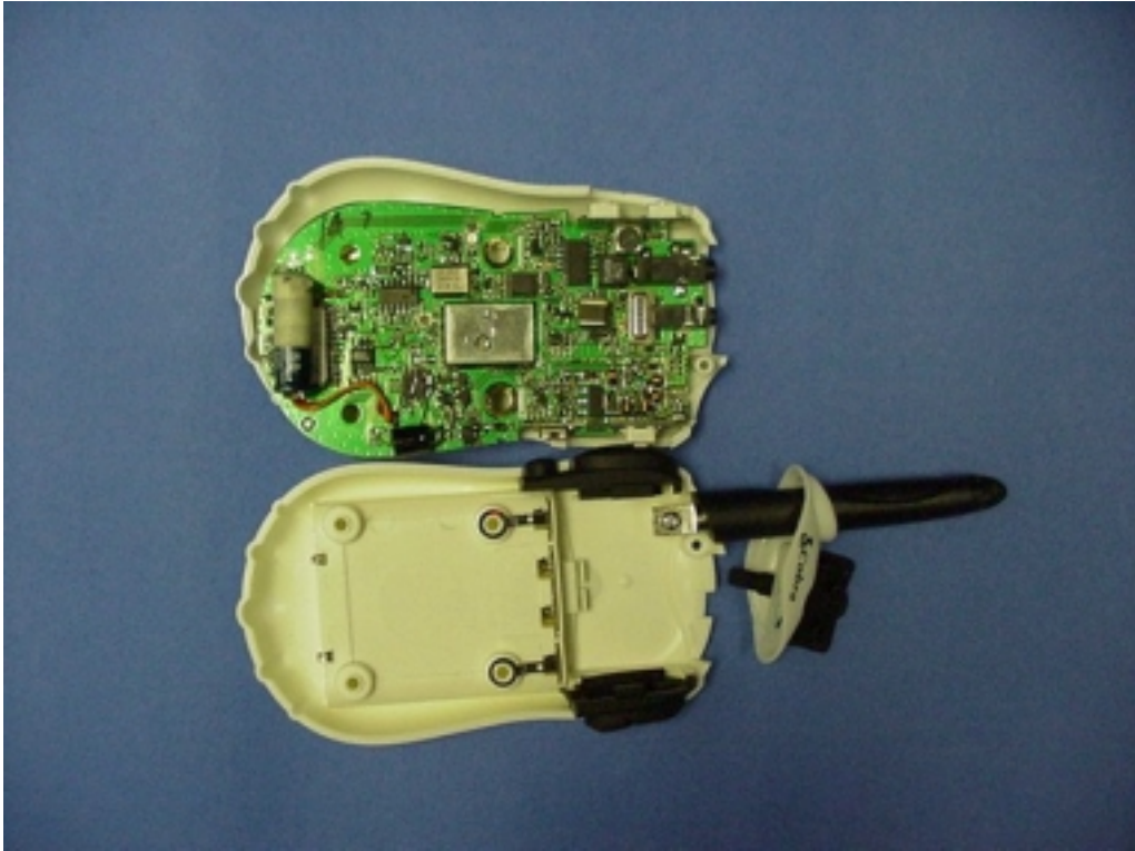
Circuit Board, Component Side
