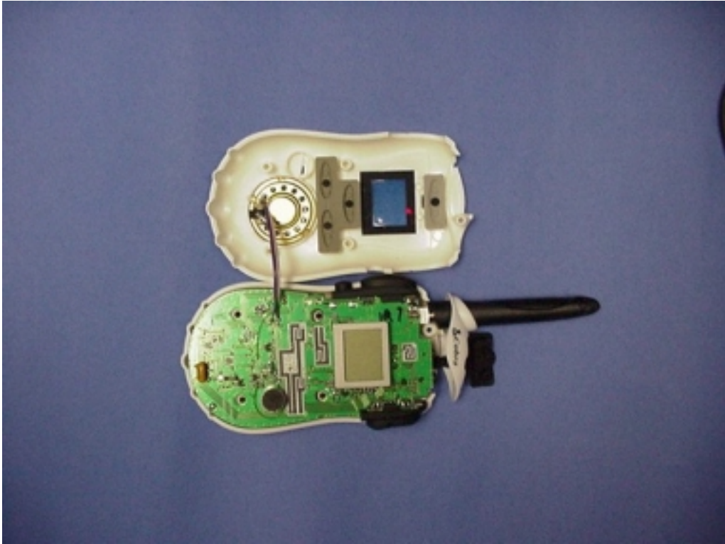
Circuit Board, Track Side
