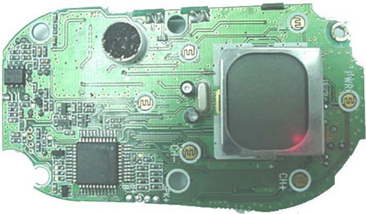
PCB Front w/o Shield
