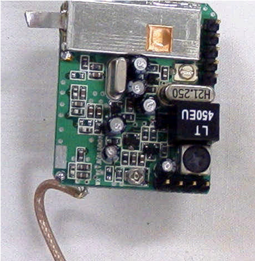
lower center board, solder side.
