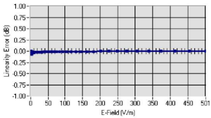
Linearity
