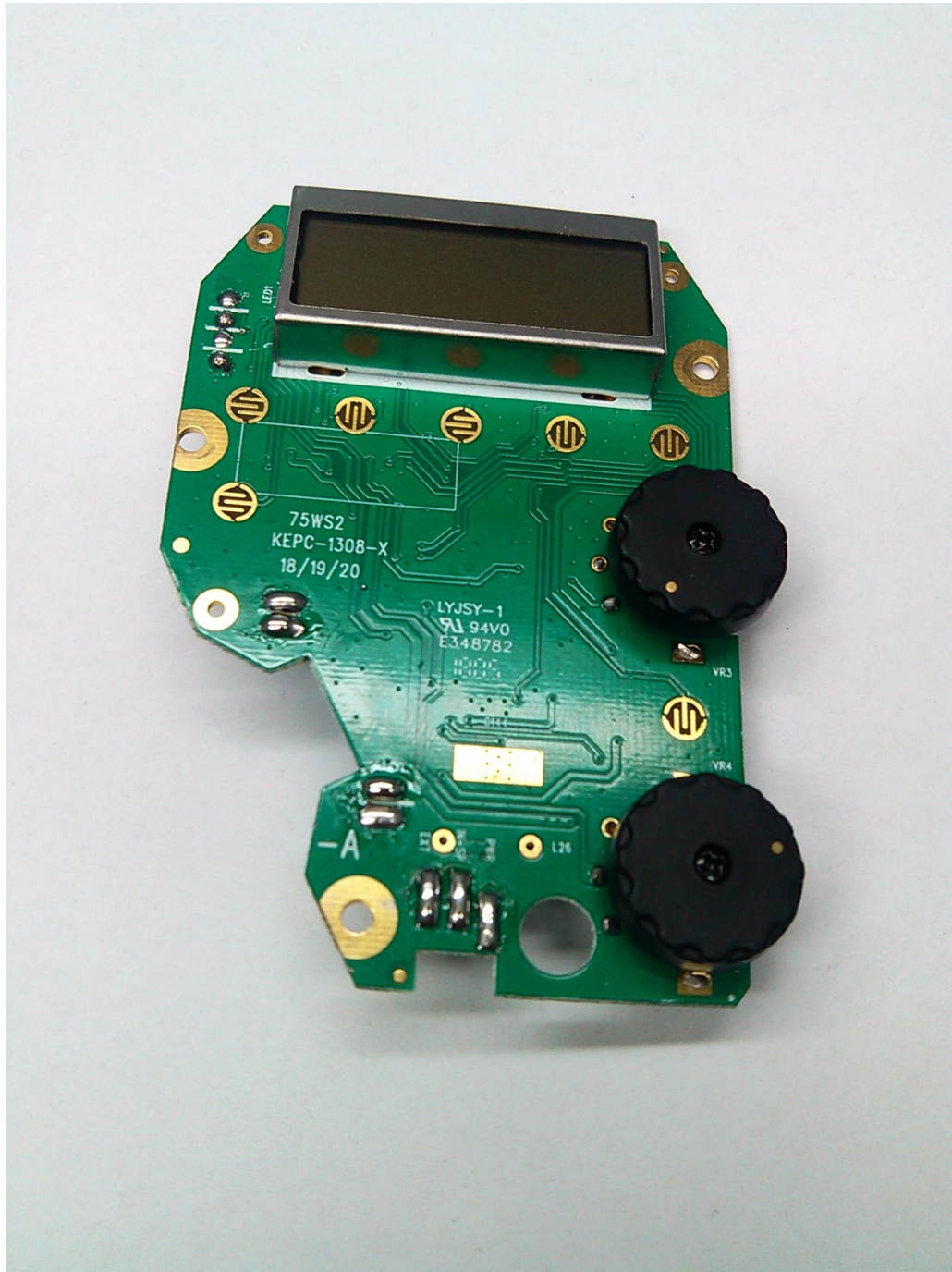
TOP PCB SIDE 1
