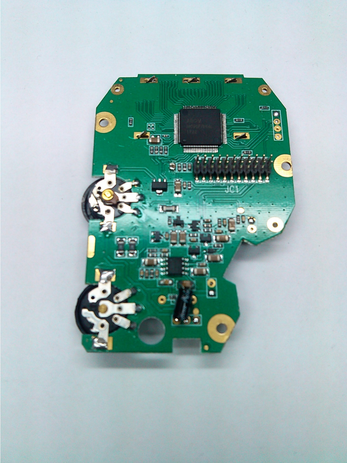
TOP PCB SIDE 2
