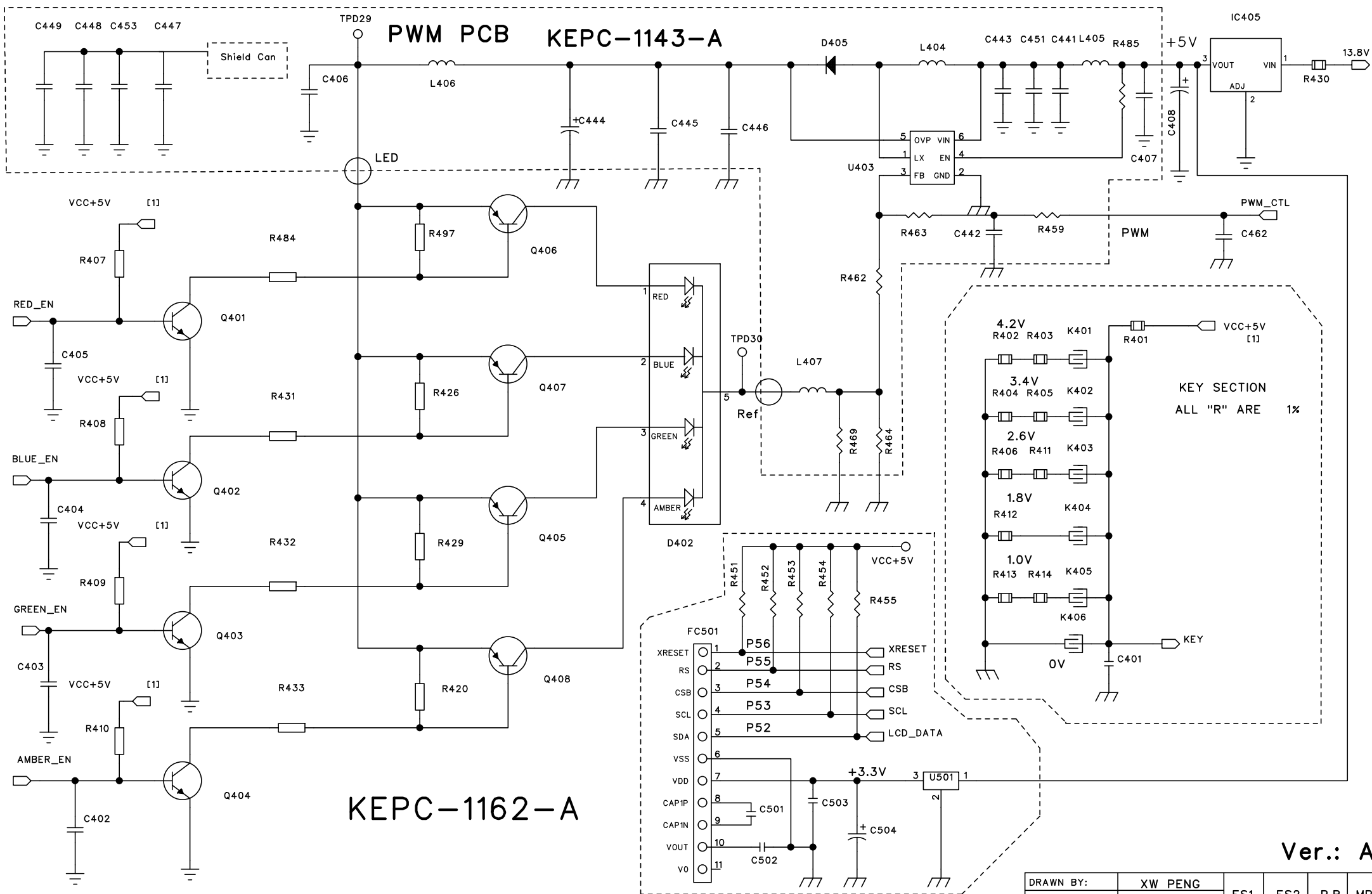
CIRCUIT DIAGRAM OF 25LX LCD
