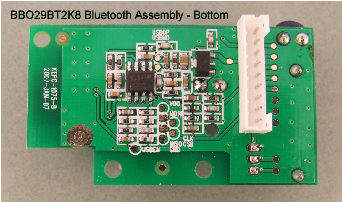
Bluetooth Assembly BBO29BT2K8
