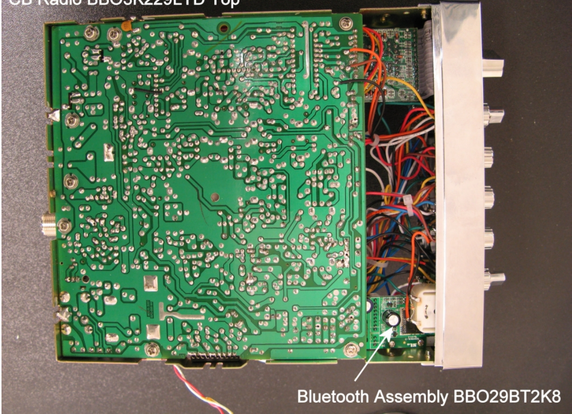
CB Radio BBO3K229LTD Top
