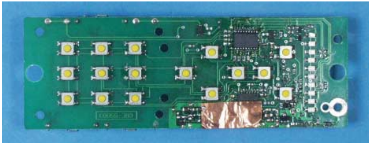
Circuit Board w/Shield
