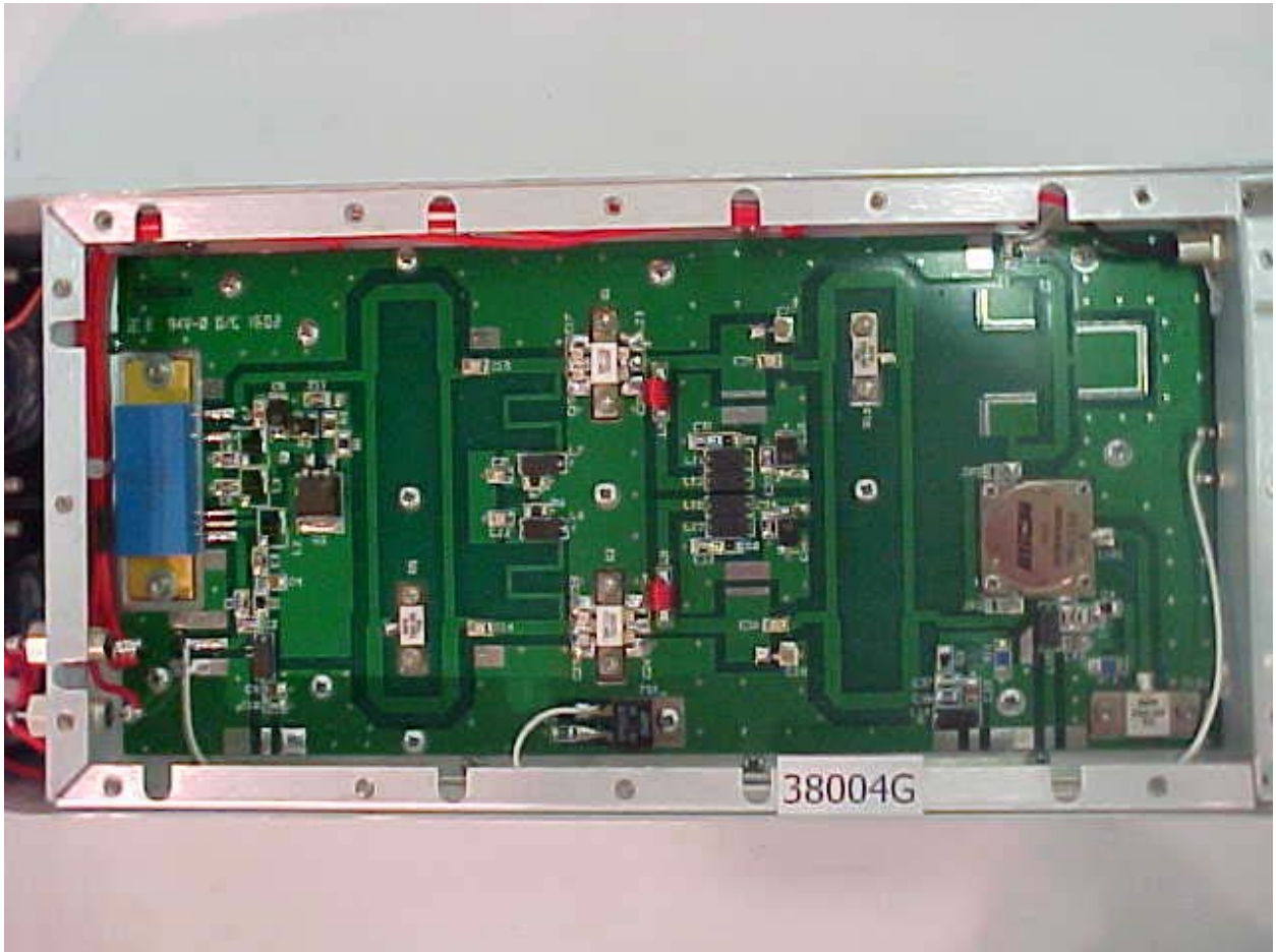
Photo 2 Detail View – Internal – Circuit Side of PCB
