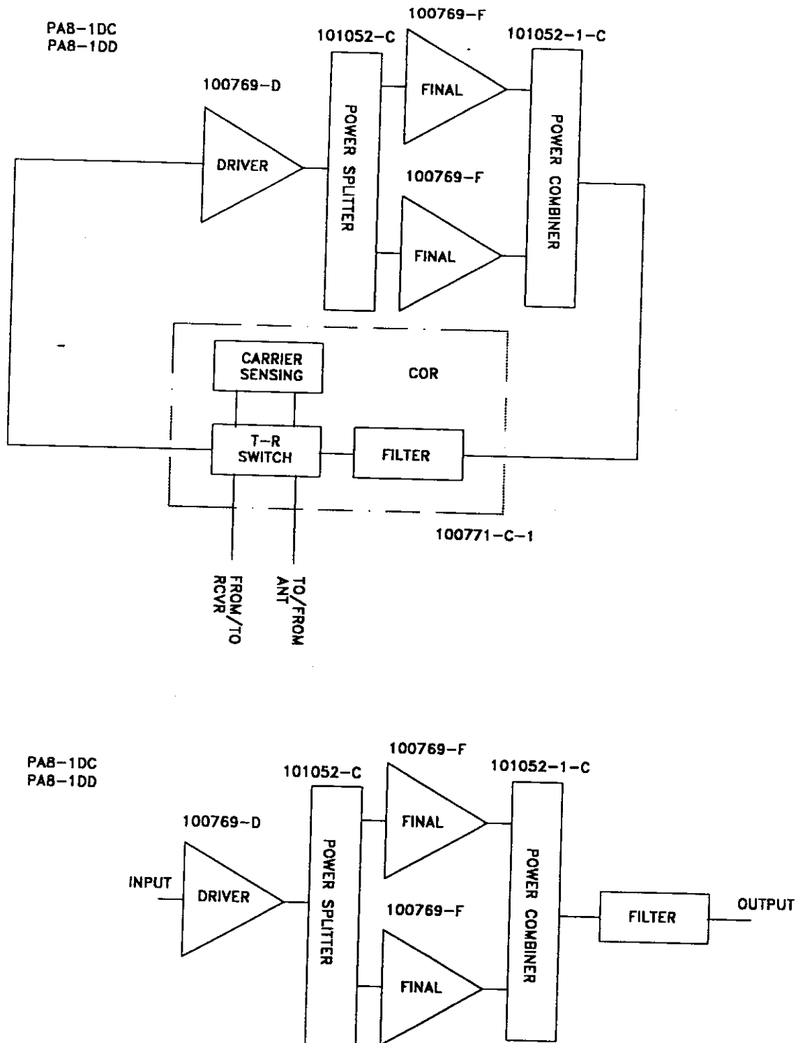
FIGURE 6 BLOCK DIAGRAMS
