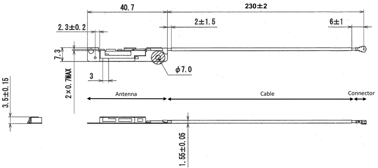
2. Wi-Fi Antenna [fig.2]
