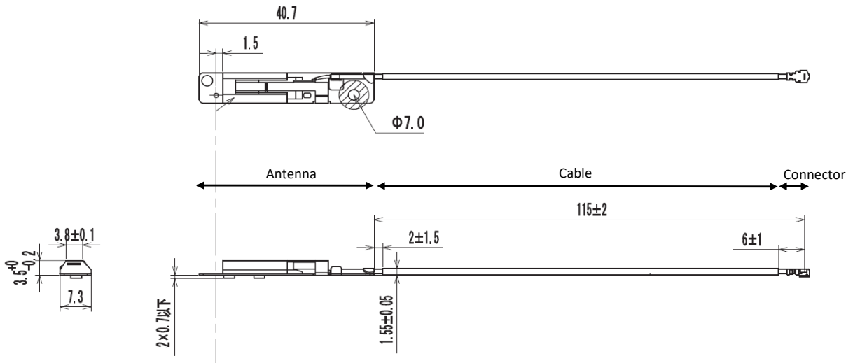
1. Bluetooth Antenna [fig.1]
