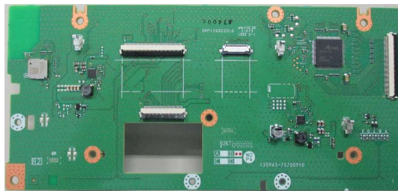
Solder side
