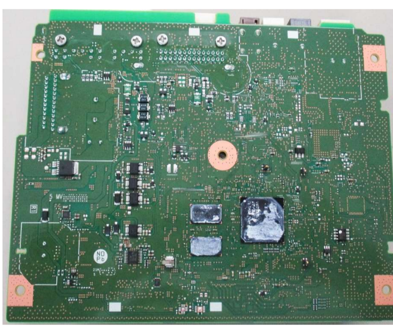
Solder side
