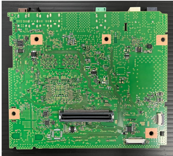
Solder side
