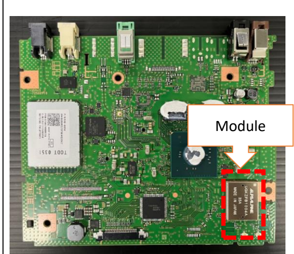
Component side
