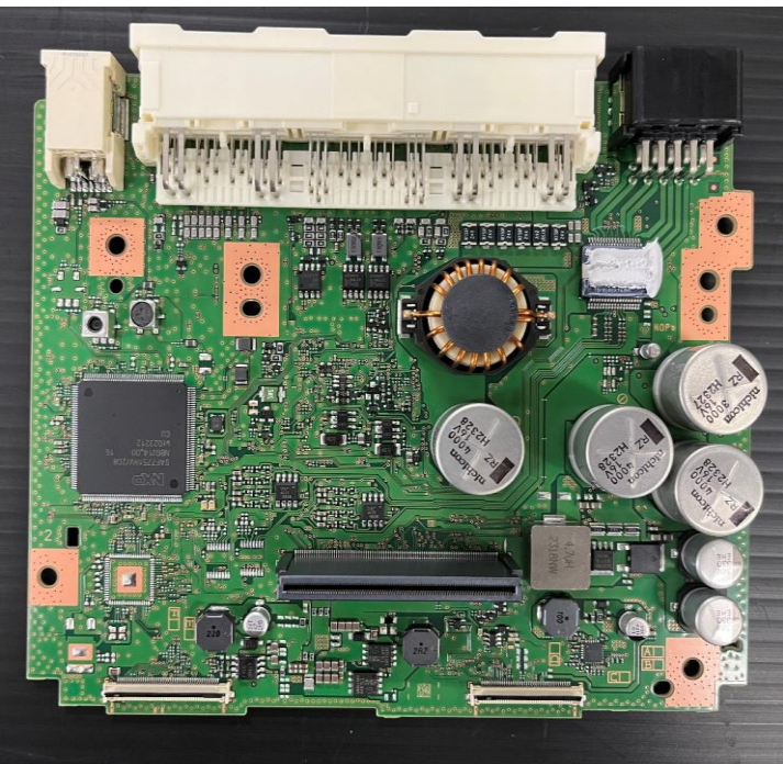
Component side
