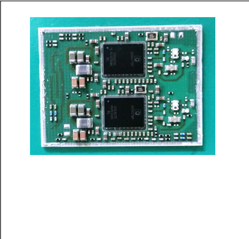
Internal Photo
