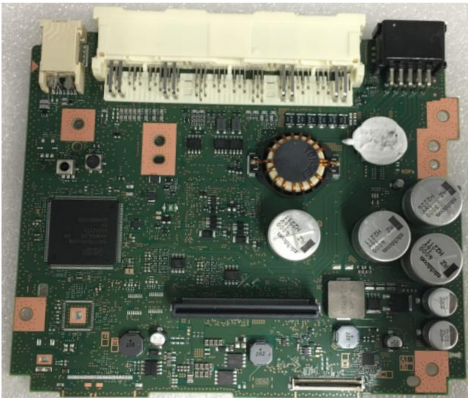
Component side
