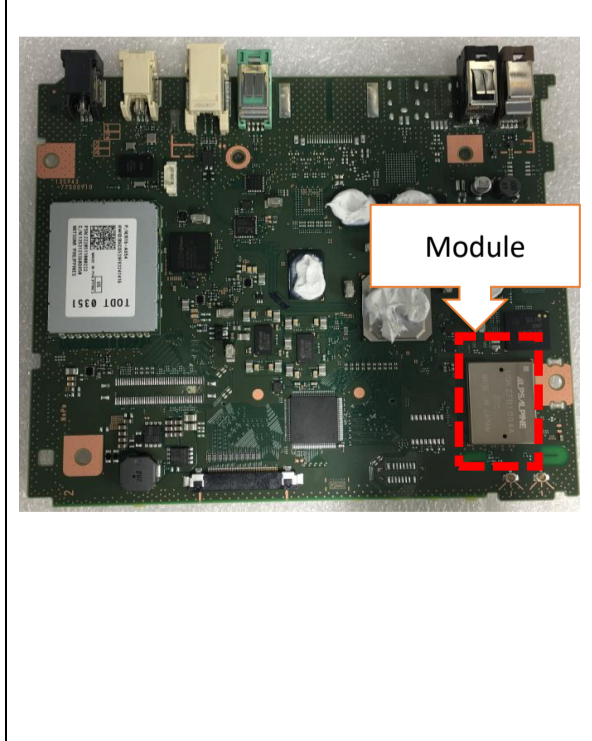
Component side
