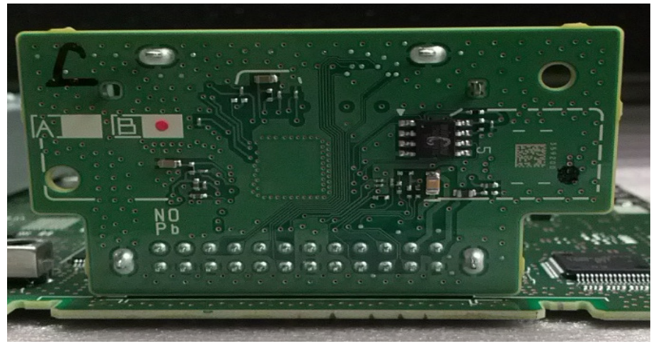
Solder side
