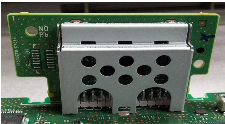
Component side
