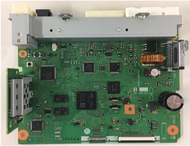
Component side
