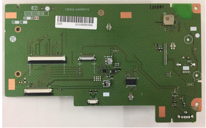
Solder side
