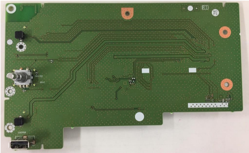
Component side
