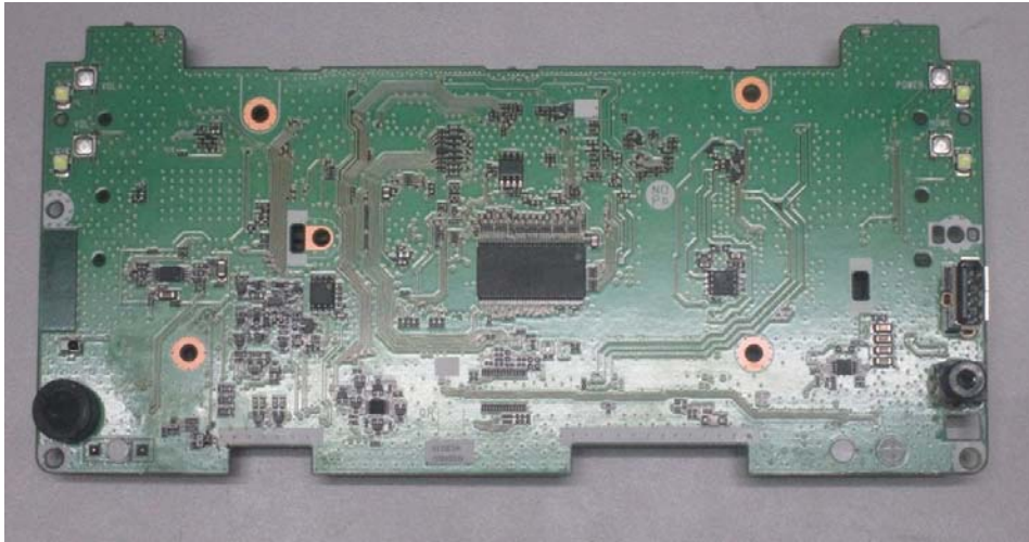
PANEL PCB ASSEMBLY (Part Side)
