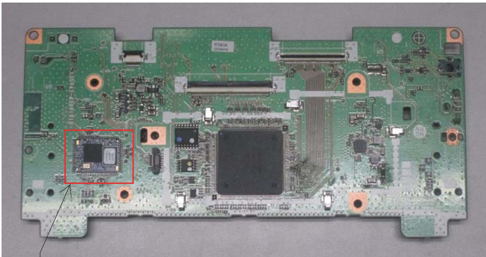
PANEL PCB ASSEMBLY (Solder Side)
