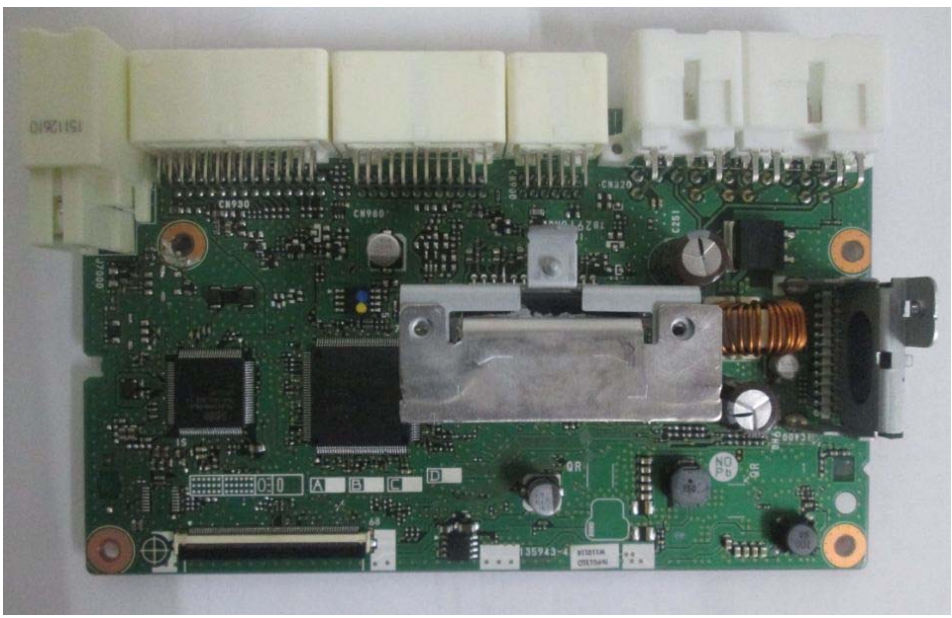
MAIN PCB ASSEMBLY (Part Side)
