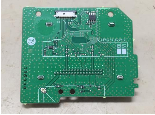
[XM Board] Component side
