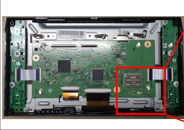
[FT0106C RF Module Position, RF Antenna Position]
