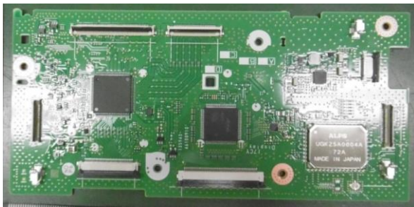
Component side
