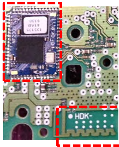
Bluetooth Antenna
