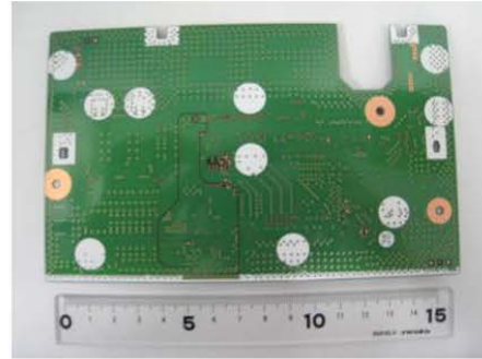
Solder side
