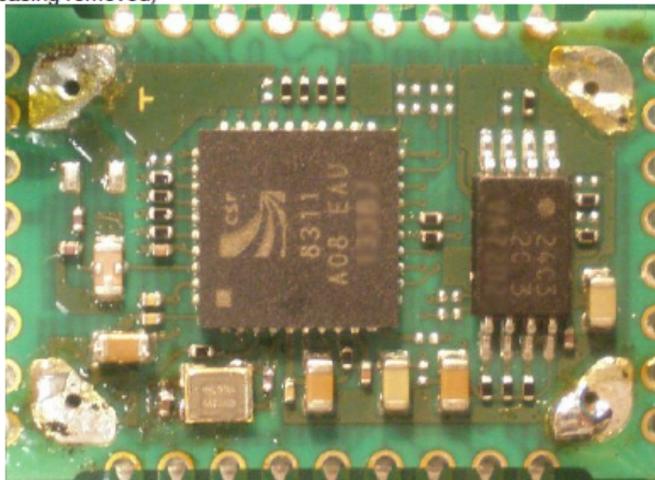
Top View – Internal (Shield casing removed)
