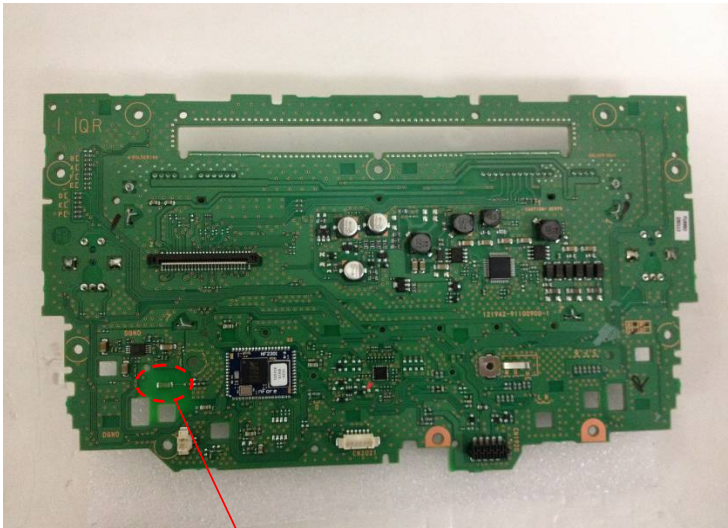
Bluetooth Antenna
