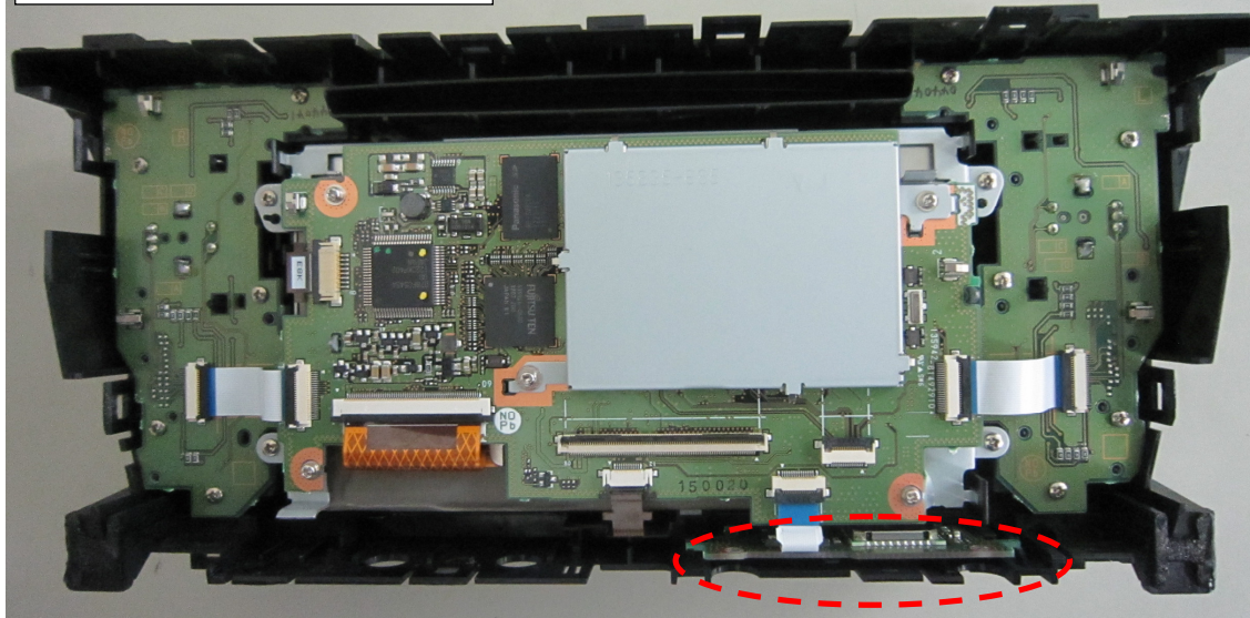
Back side of front panel
