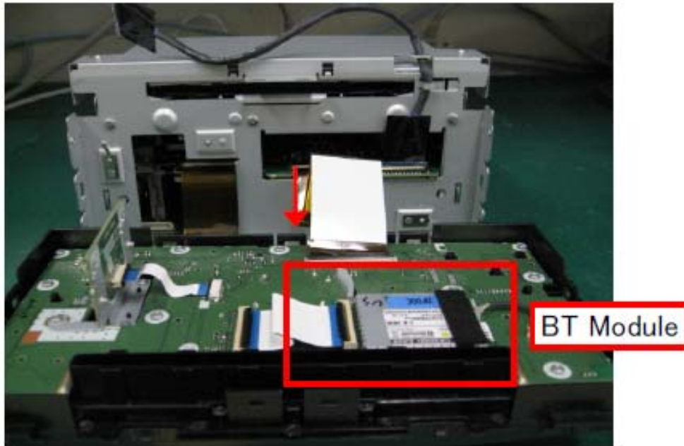
Location of Bluetooth module
