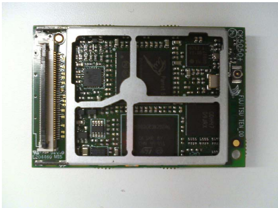
Bluetooth module (without shielded cover)
