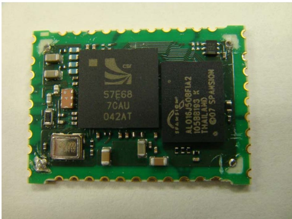
Bluetooth module (without shielded cover)
