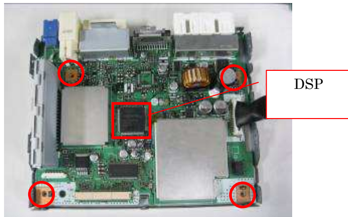
Audio PCB (4 screws)
