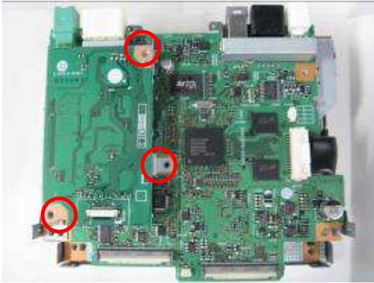
Deck PCB (3 screws)
