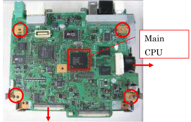
CPU PCB (4 screws)
