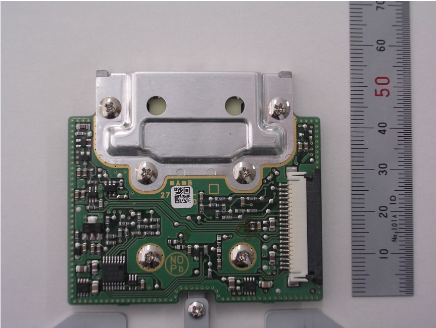
RF-unit parts-side
