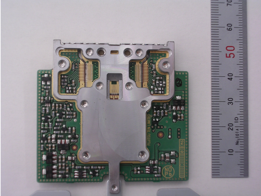
RF-unit solder-side
