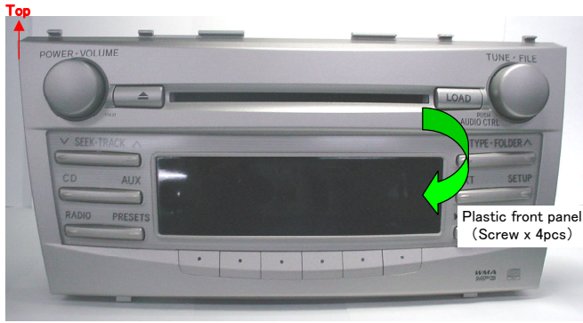
Front panel is dismantled
