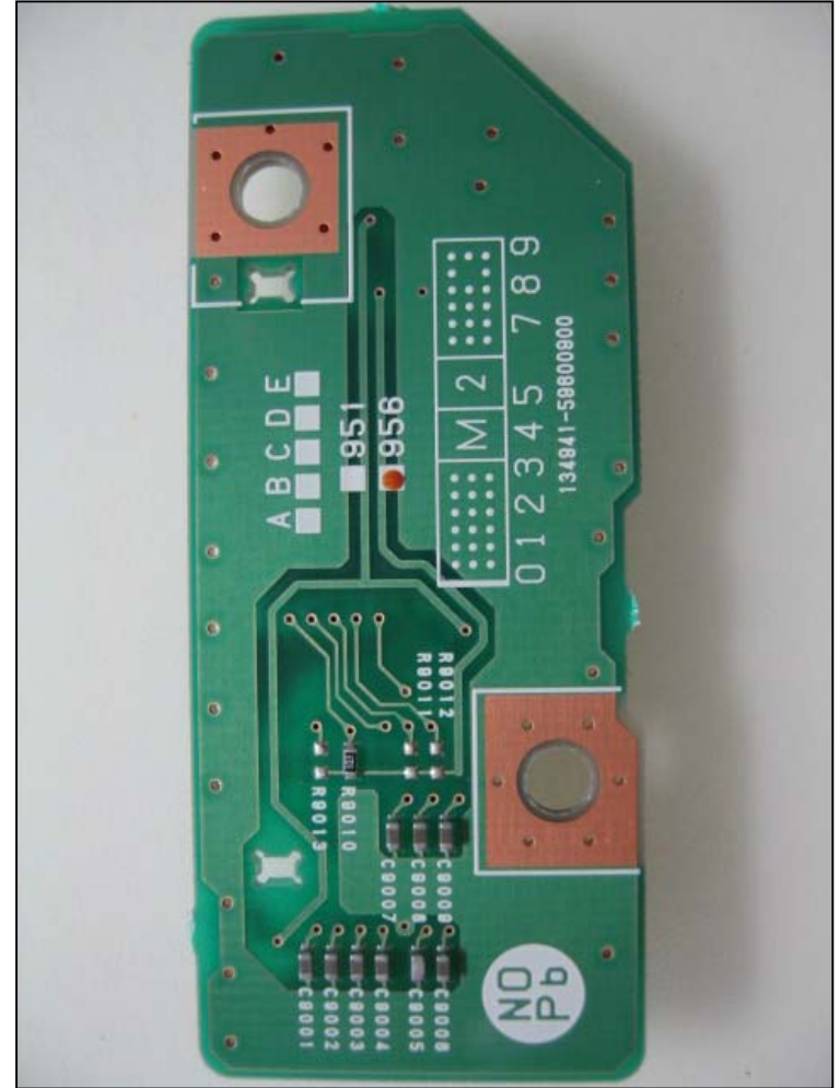
Solder side
