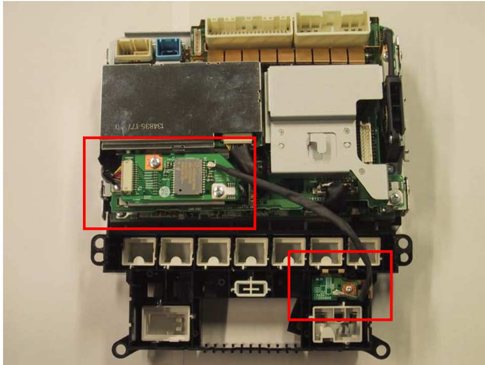
Location of BT module and Antenna
