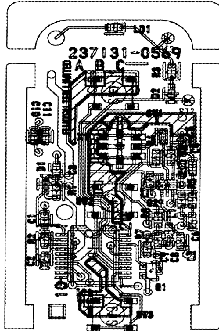
OLD Circuit
