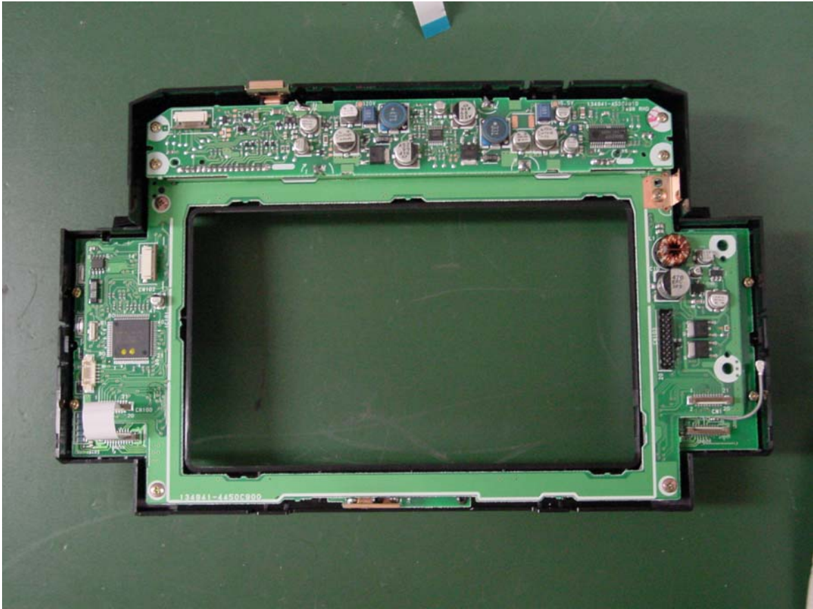
PCB without BT module
