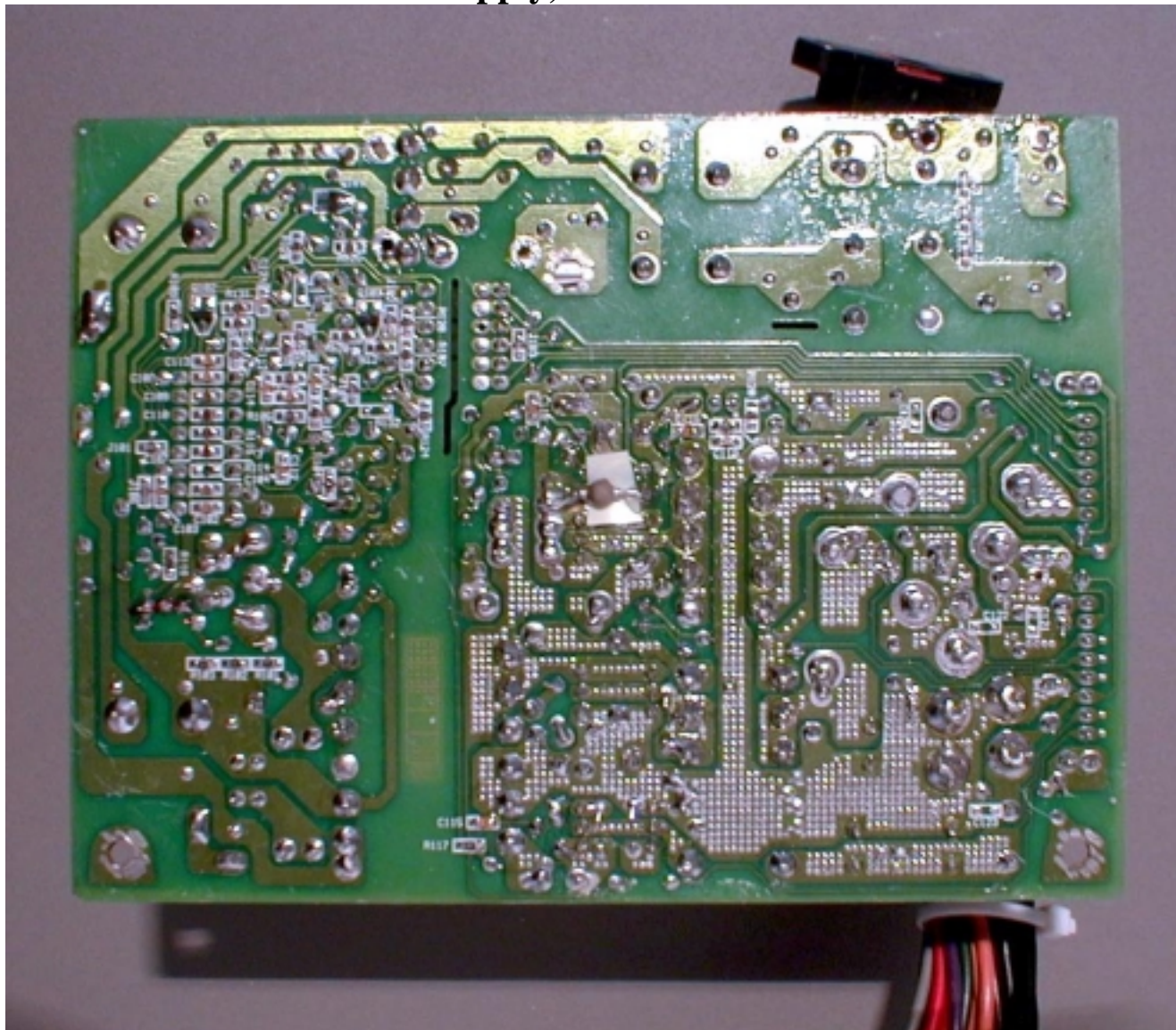
12 – Power supply, daughter board foil side view
