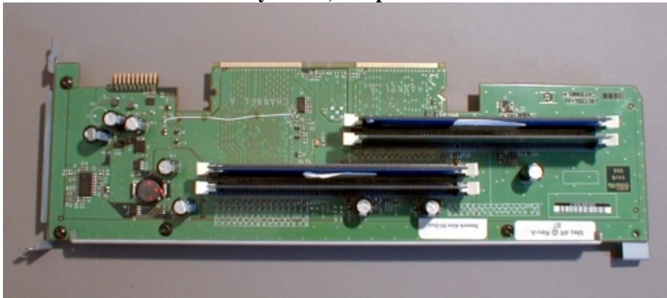
19 – Memory board, component side view
