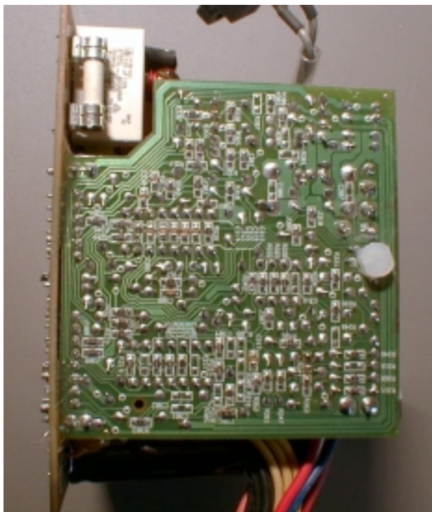
12 – Power supply, daughter board foil side view
