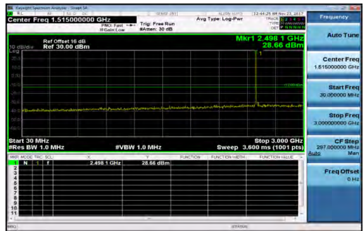
30MHz-3GHz_Band41_5MHz_QPSK_1_0_LowCH39675
