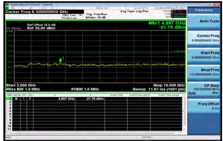
3GHz-10GHz_Band26_3MHz_OPSK_1_0_MidCH26740
