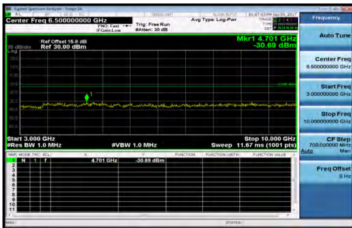
3GHz-10GHz_Band26_15MHz_OPSK_1_0_HighCH26965-841.5
