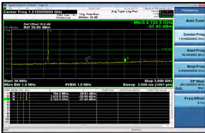
30MHz-3GHz_Band12_10MHz_QPSK_1_0_MidCH23095-707.5
