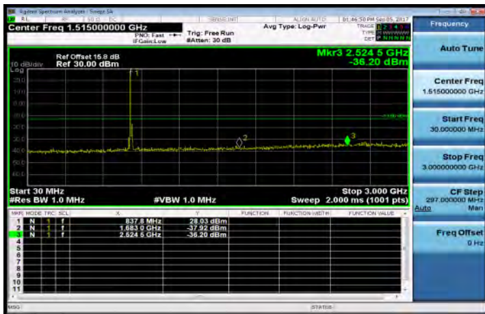
30MHz-3GHz_Band26_15MHz_OPSK_1_0_HighCH26965-841.5
