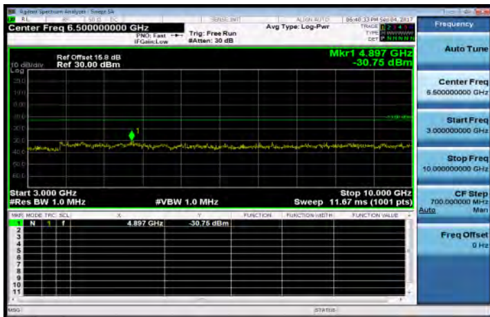
3GHz-10GHz_Band12_10MHz_QPSK_1_0_LowCH23060-704
