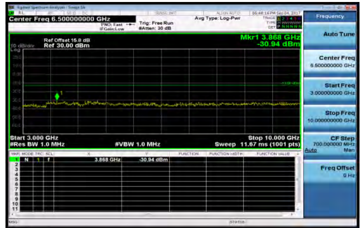
3GHz-10GHz_Band12_5MHz_QPSK_1_0_MidCH23095-707.5
