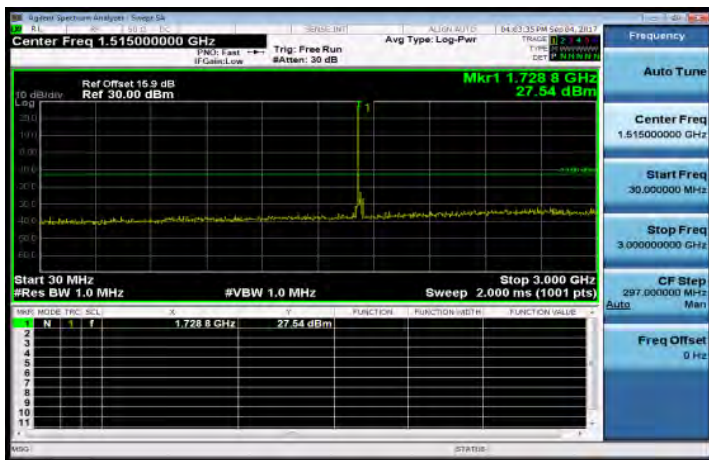
30MHz-3GHz_Band4_15MHz_QPSK_1_0_MidCH20175-1732.5
