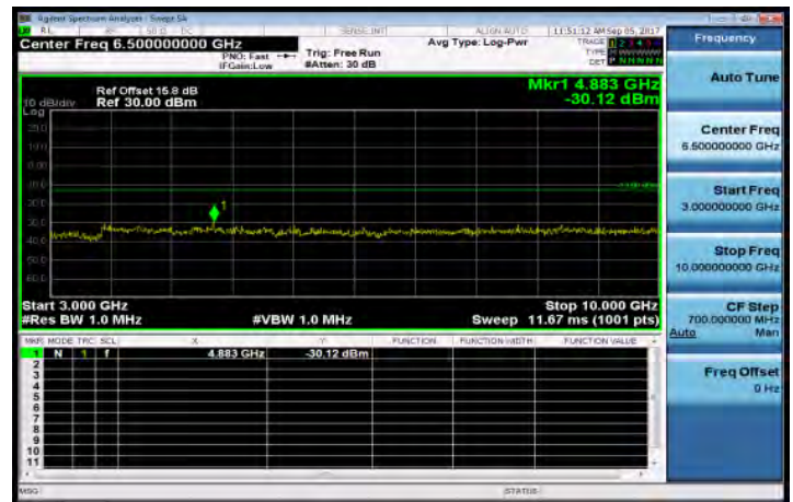
3GHz-10GHz_Band26_3MHz_QPSK_1_0_LowCH26705-815.5
