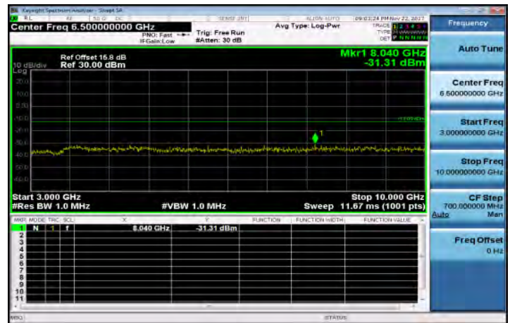
3GHz-10GHz_Band17_10MHz_QPSK_1_0_LowCH23780-709
