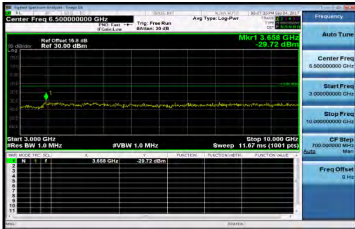
3GHz-10GHz_Band5_5MHz_QPSK_1_0_LowCH20425-826.5
