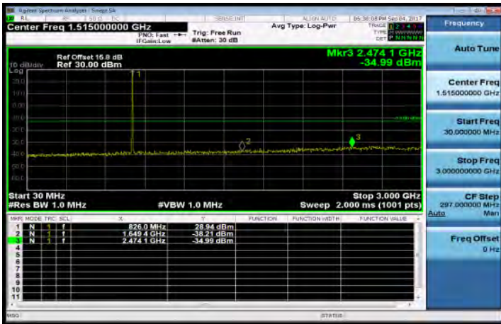
30MHz-3GHz_Band5_1_4MHz_QPSK_1_0_LowCH20407-824.7
