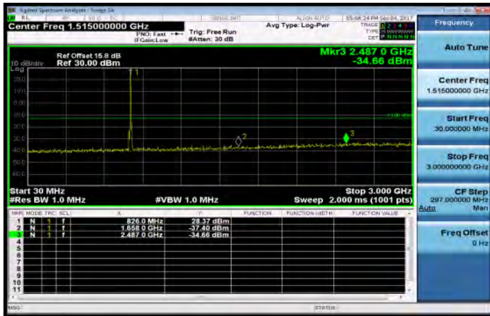
30MHz-3GHz_Band5_10MHz_QPSK_1_0_LowCH20450-829
