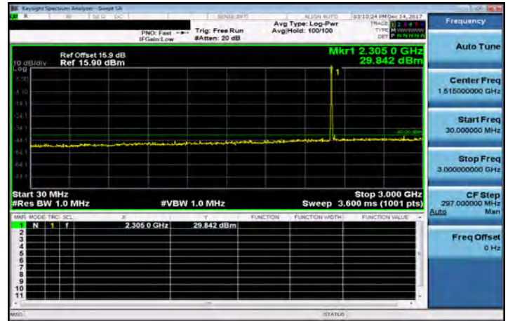
30MHz-3GHz_Band30_5MHz_OPSK_1_0_LowCH27685
