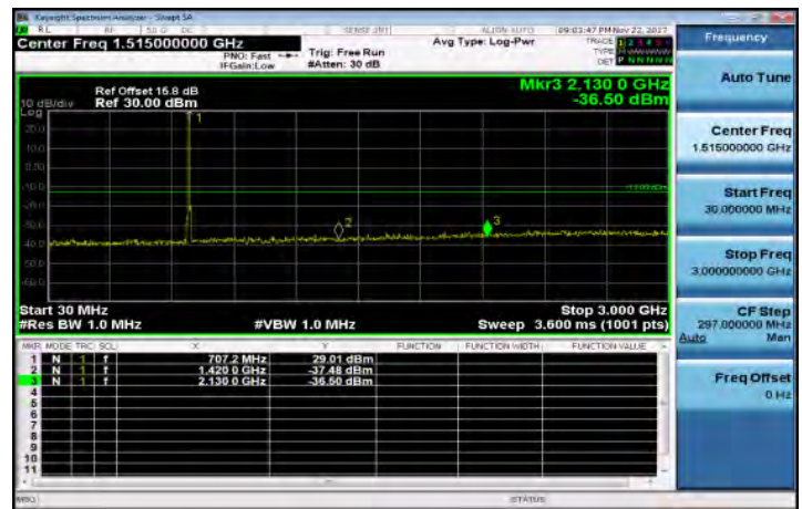
30MHz-3GHz_Band17_10MHz_QPSK_1_0_MidCH23790-710
