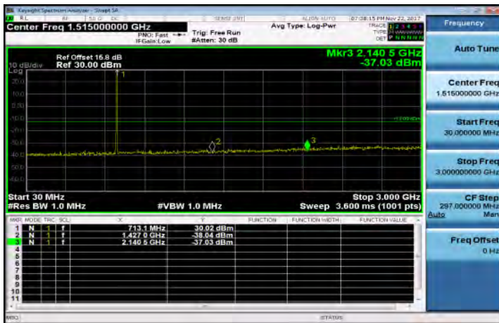
30MHz-3GHz_Band17_5MHz_QPSK_1_0_HighCH23825-713.5
