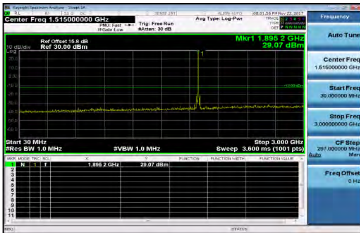
30MHz-3GHz_Band25_20MHz_QPSK_1_0_HighCH26590-1905
