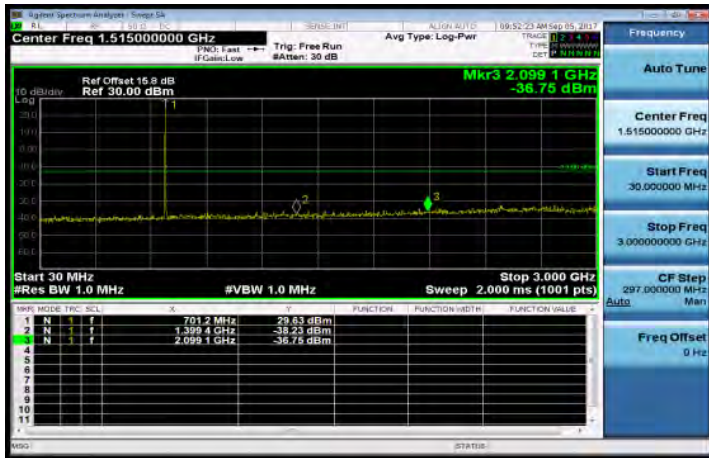
30MHz-3GHz_Band12_1_4MHz_QPSK_1_0_LowCH23017-699.7
