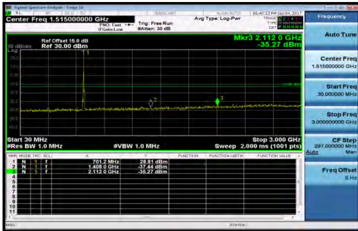
30MHz-3GHz_Band12_10MHz_QPSK_1_0_LowCH23060-704
