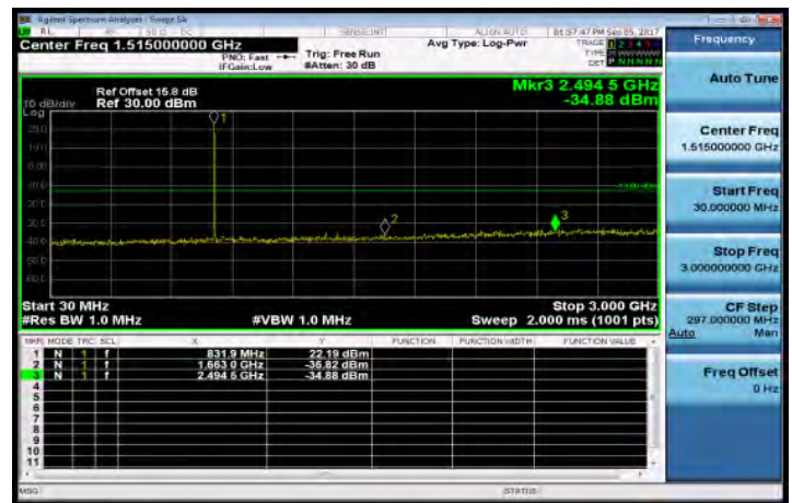
30MHz-3GHz_Band26_1_4MHz_QPSK_1_0_MidCH26865-831.5
