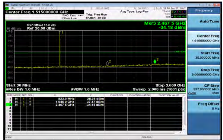
30MHz-3GHz_Band26_3MHz_OPSK_1_0_HighCH26775
