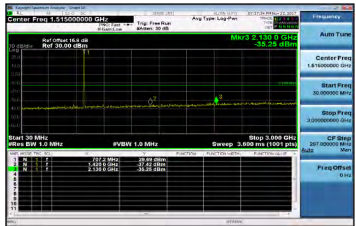
30MHz-3GHz_Band17_5MHz_QPSK_1_0_MidCH23790-710
