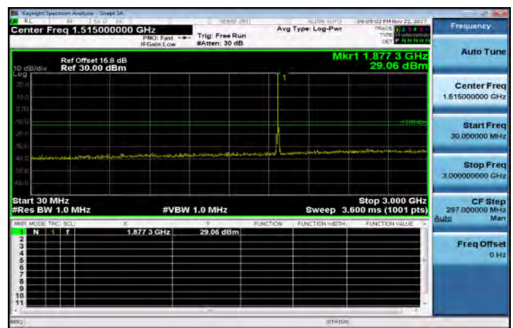
30MHz-3GHz_Band25_10MHz_QPSK_1_0_MidCH26365-1882.5
