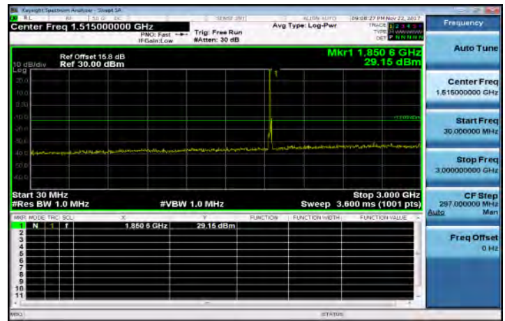
30MHz-3GHz_Band25_10MHz_QPSK_1_0_LowCH26090-1855
