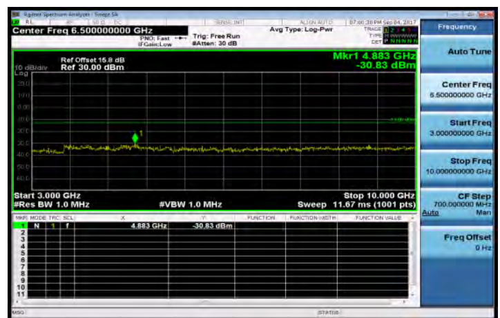
3GHz-10GHz_Band12_3MHz_QPSK_1_0_HighCH23165-714.5
