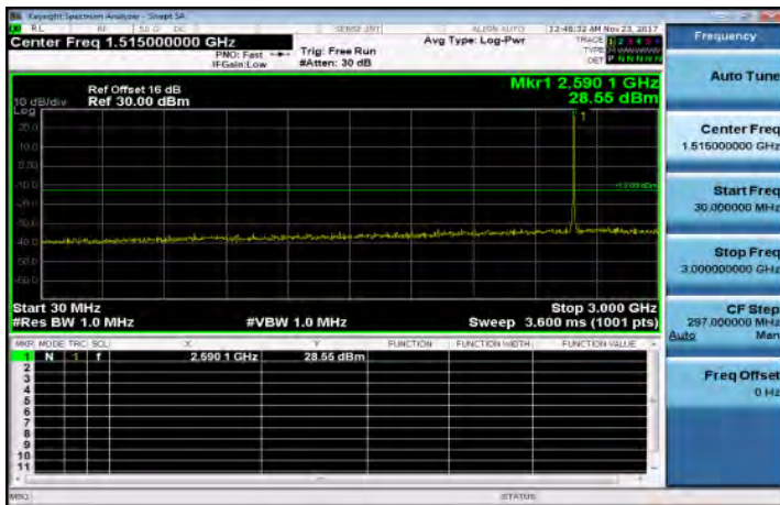
30MHz-3GHz_Band41_5MHz_QPSK_1_0_MidCH40620
