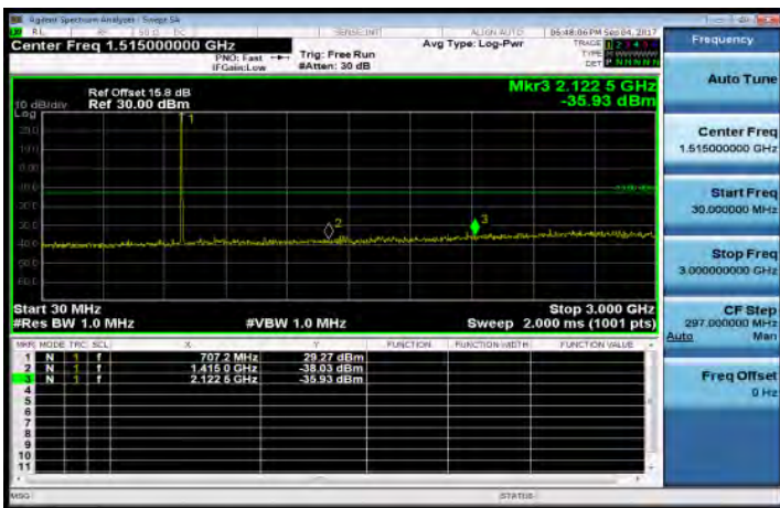
30MHz-3GHz_Band12_5MHz_QPSK_1_0_MidCH23095-707.5
