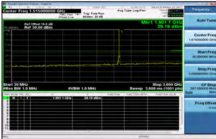
30MHz~3GHz_Band25_15MHz_QPSK_1_0_HighCH26615-1907.5
