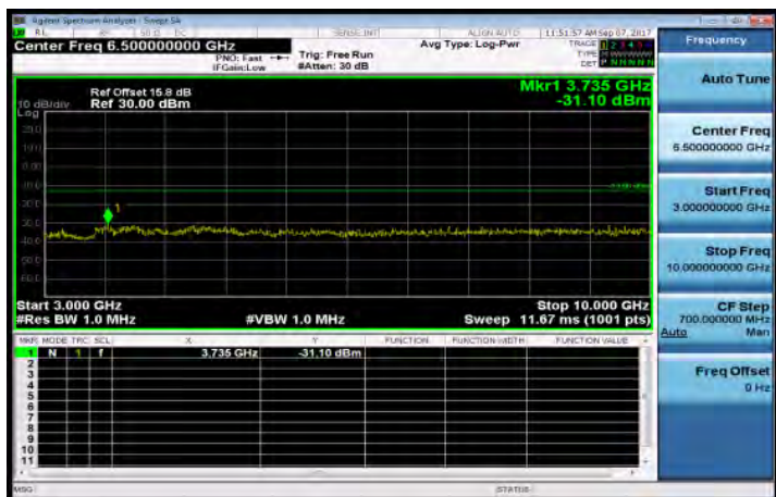
3GHz-10GHz_Band26_5MHz_OPSK_1_0_LowCH26715
