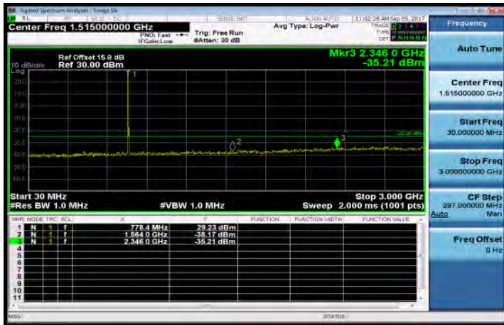
30MHz-3GHz_Band13_10MHz_QPSK_1_0_LowCH23230-782
