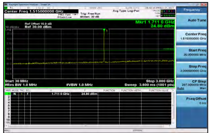
30MHz-3GHz_Band66_1_4MHz_QPSK_1_0_LowCH131979
