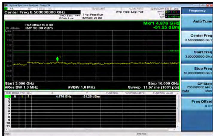
3GHz-10GHz_Band26_5MHz_OPSK_1_0_HighCH2675
