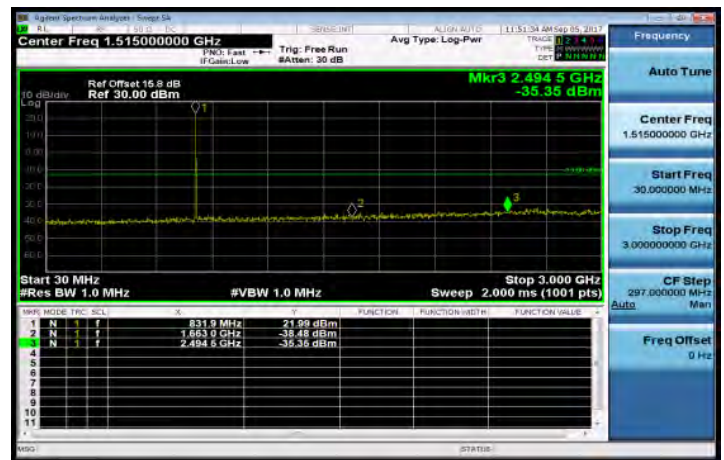
30MHz-3GHz_Band26_3MHz_QPSK_1_0_MidCH26865-831.5
