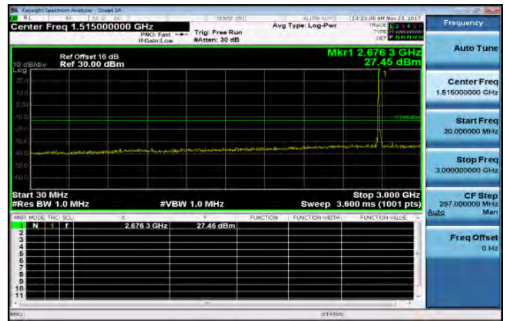
30MHz-3GHz_Band41_15MHz_QPSK_1_0_HighCH41515
