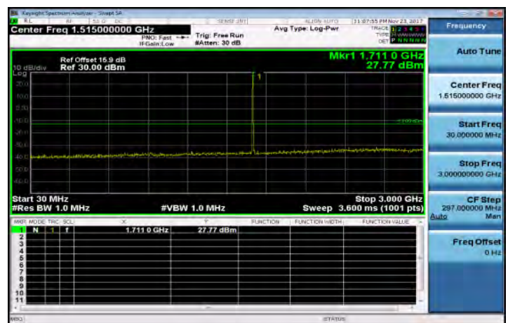
30MHz-3GHz_Band66_3MHz_QPSK_1_0_LowCH131987
