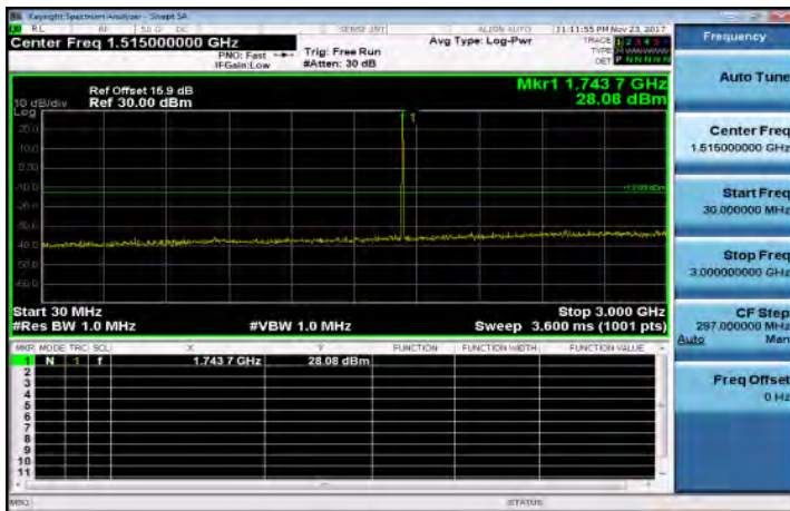
30MHz-3GHz_Band66_3MHz_QPSK_1_0_MidCH132322
