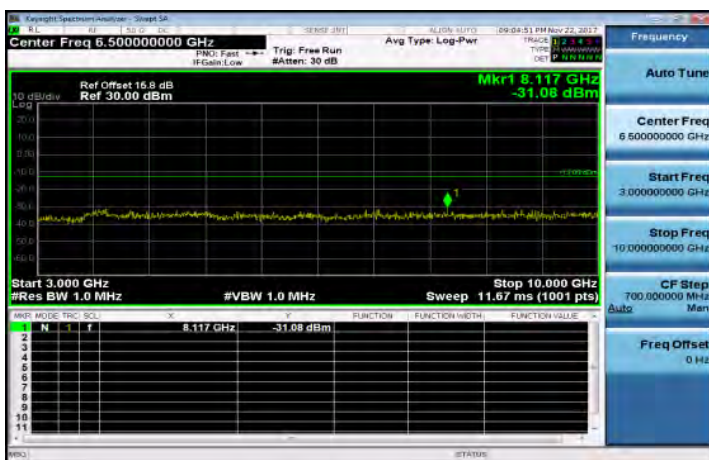
3GHz-10GHz_Band17_10MHz_QPSK_1_0_HighCH23800-711
