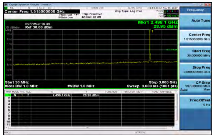
30MHz-3GHz_Band41_15MHz_QPSK_1_0_LowCH39725
