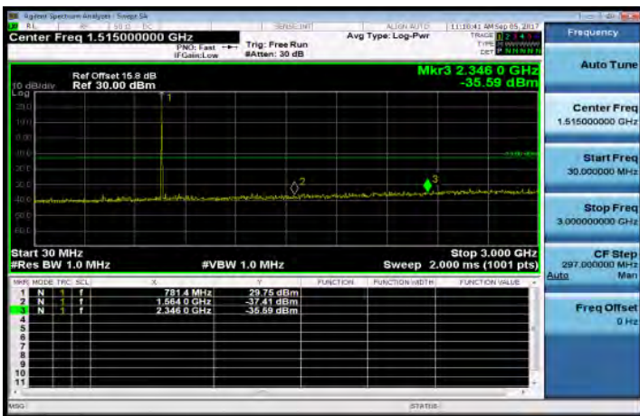
30MHz-3GHz_Band13_5MHz_QPSK_1_0_MidCH23230-782
