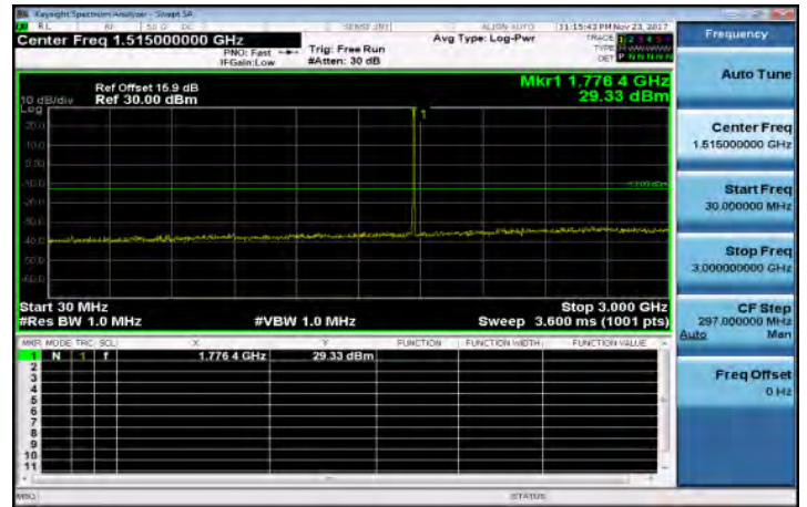
30MHz-3GHz_Band66_3MHz_QPSK_1_0_HighCH132657
