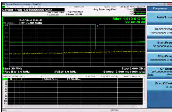
30MHz-3GHz_Band25_5MHz_QPSK_1_0_HighCH26665-1912.5
