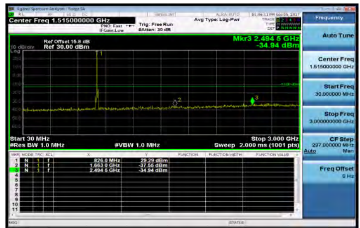
30MHz-3GHz_Band26_15MHz_QPSK_1_0_MidCH26865-831.5
