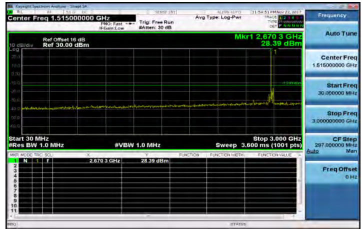
30MHz-3GHz_Band41_20MHz_QPSK_1_0_HighCH41490
