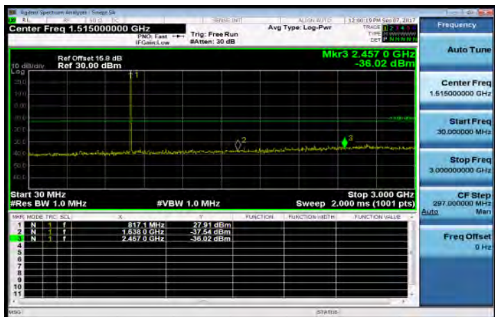
30MHz-3GHz_Band26_5MHz_OPSK_1_0_MidCH26740
