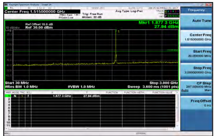
30MHz-3GHz_Band25_15MHz_QPSK_1_0_MidCH26365-1882.5
