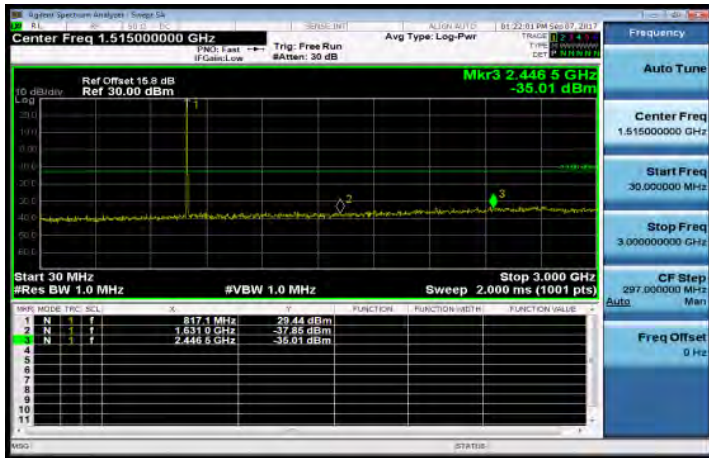
30MHz-3GHz_Band26_3MHz_OPSK_1_0_LowCH26705
