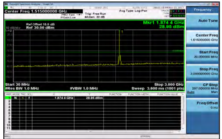
30MHz~3GHz_Band25_20MHz_QPSK_1_0_MidCH26365-1882.5
