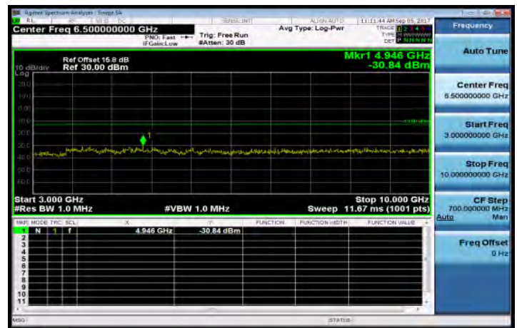
3GHz-10GHz_Band13_5MHz_QPSK_1_0_HighCH23255-784.5
