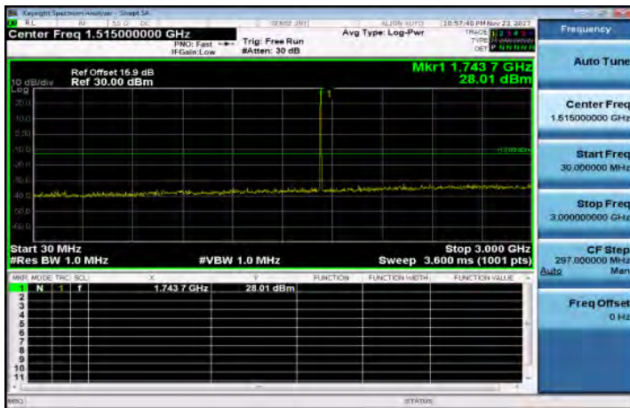
30MHz-3GHz_Band66_5MHz_QPSK_1_0_MidCH132322
