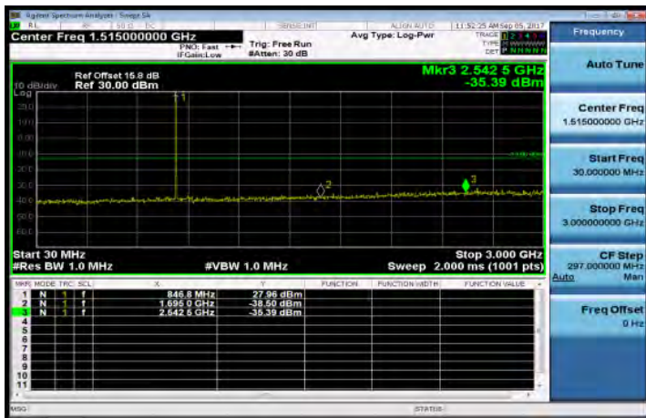
30MHz-3GHz_Band26_3MHz_QPSK_1_0_HighCH27025-847.5
