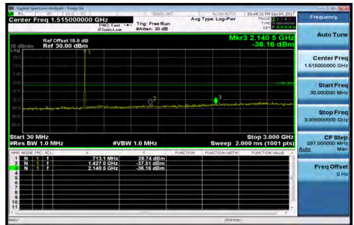
30MHz-3GHz_Band12_5MHz_QPSK_1_0_HighCH23155-713.5
