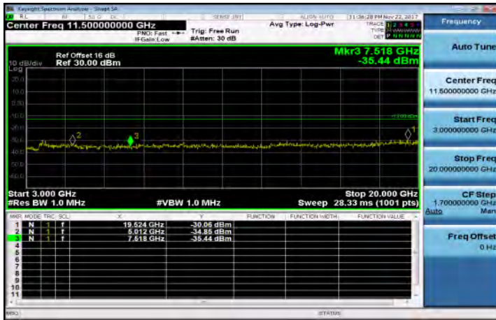
3GHz-10GHz_Band41_20MHz_QPSK_1_0_LowCH39750
