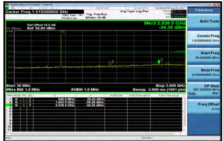
30MHz-3GHz_Band5_5MHz_QPSK_1_0_HighCH20625-846.5
