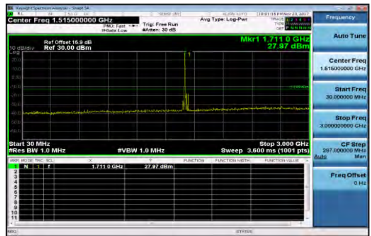
30MHz~3GHz_Band66_20MHz_QPSK_1_0_LowCH132072
