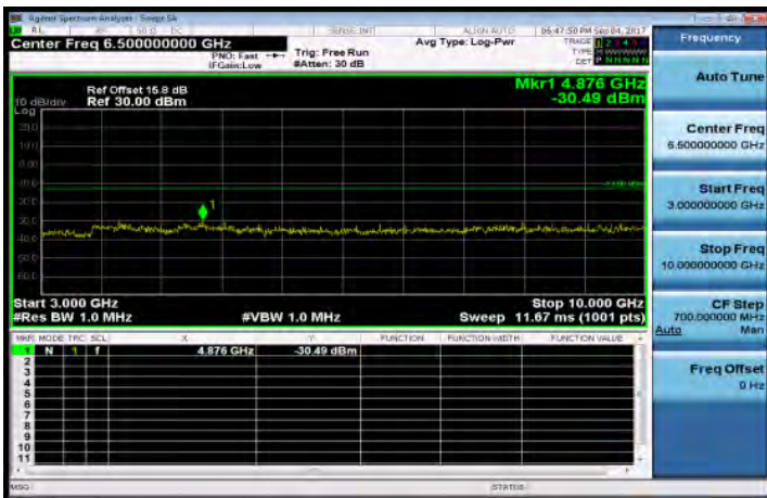
3GHz-10GHz_Band12_5MHz_QPSK_1_0_LowCH23035-701.5
