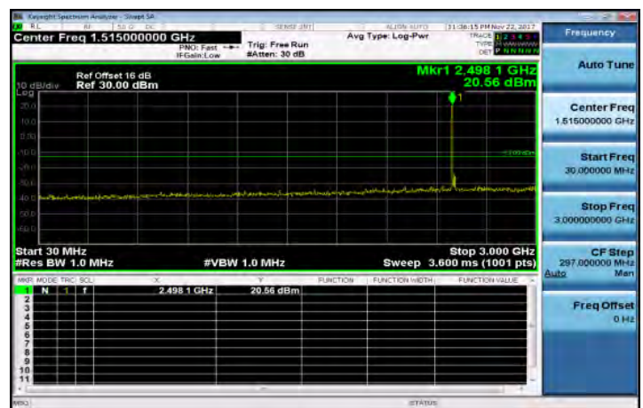
30MHz-3GHz_Band41_20MHz_QPSK_1_0_LowCH39750
