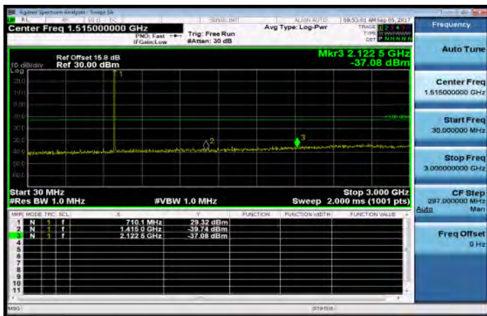
30MHz-3GHz_Band12_1_4MHz_QPSK_1_0_MidCH23095-707.5
