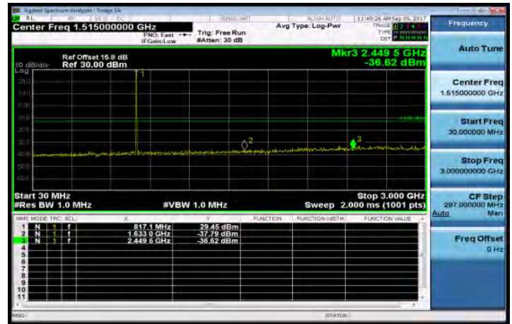
30MHz-3GHz_Band26_5MHz_QPSK_1_0_LowCH26715-816.5
