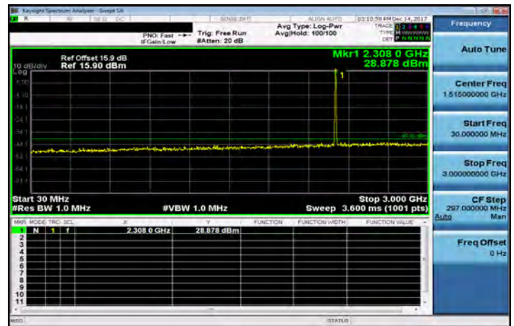
30MHz-3GHz_Band30_5MHz_OPSK_1_0_MidCH27710
