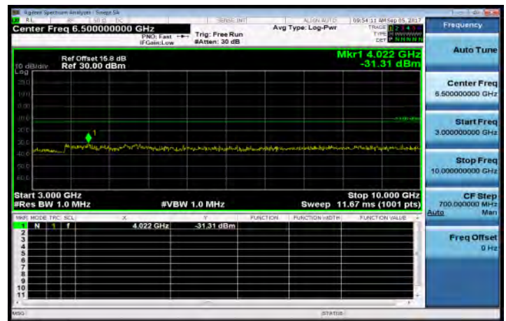
3GHz-10GHz_Band12_1_4MHz_QPSK_1_0_HighCH23173-715.3
