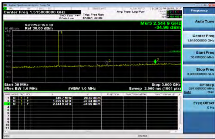
30MHz-3GHz_Band26_1_4MHz_QPSK_1_0_HighCH27033-848.3
