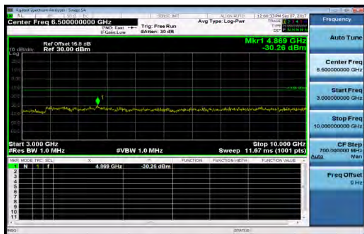
3GHz-10GHz_Band26_5MHz_OPSK_1_0_MidCH26740
