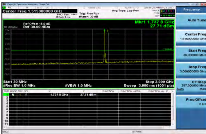
30MHz~3GHz_Band66_15MHz_QPSK_1_0_MidCH132322
