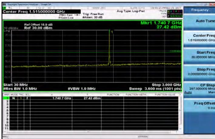
30MHz~3GHz_Band66_10MHz_QPSK_1_0_MidCH132322
