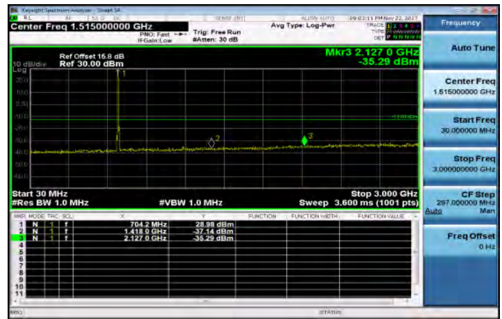
30MHz-3GHz_Band17_10MHz_QPSK_1_0_LowCH23780-709
