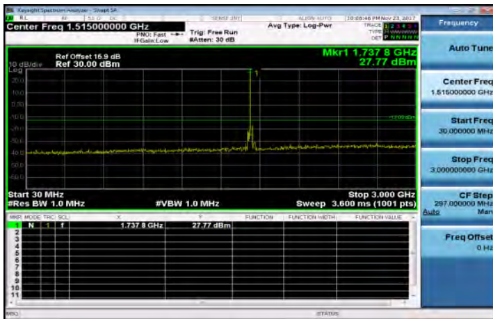
30MHz~3GHz_Band66_20MHz_QPSK_1_0_MidCH132322
