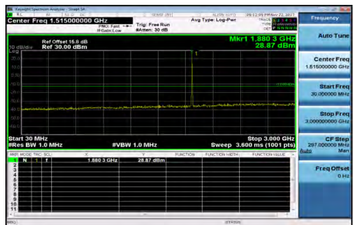
30MHz-3GHz_Band25_5MHz_OPSK_1_0_MidCH26365-1882.5
