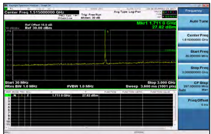
30MHz-3GHz_Band66_10MHz_QPSK_1_0_LowCH132022
