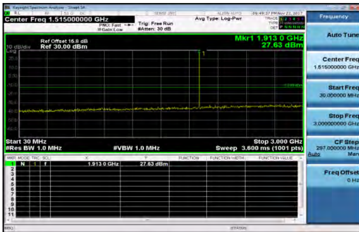
30MHz-3GHz_Band25_1_4MHz_OPSK_1_0_HighCH26683-1914.3
