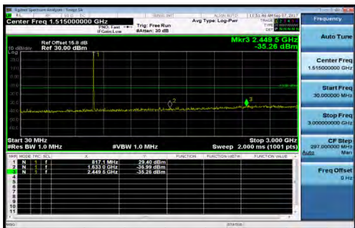
30MHz-3GHz_Band26_5MHz_OPSK_1_0_LowCH26715
