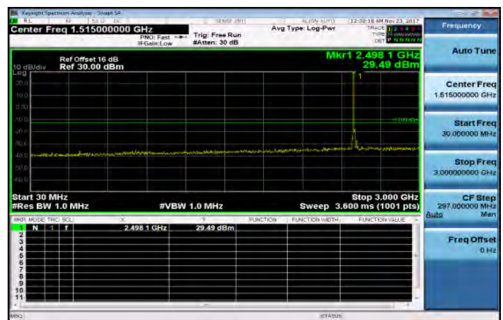
30MHz-3GHz_Band41_10MHz_QPSK_1_0_LowCH39700
