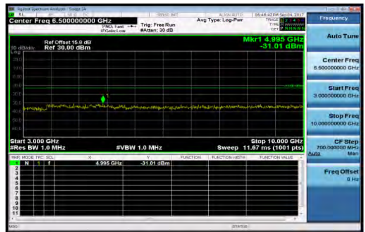
3GHz-10GHz_Band12_5MHz_QPSK_1_0_HighCH23155-713.5
