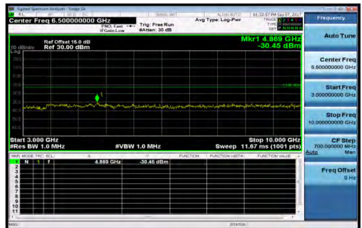
3GHz-10GHz_Band26_3MHz_OPSK_1_0_HighCH26775
