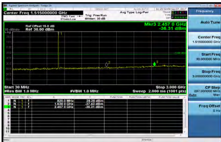
30MHz-3GHz_Band26_3MHz_OPSK_1_0_MidCH26740
