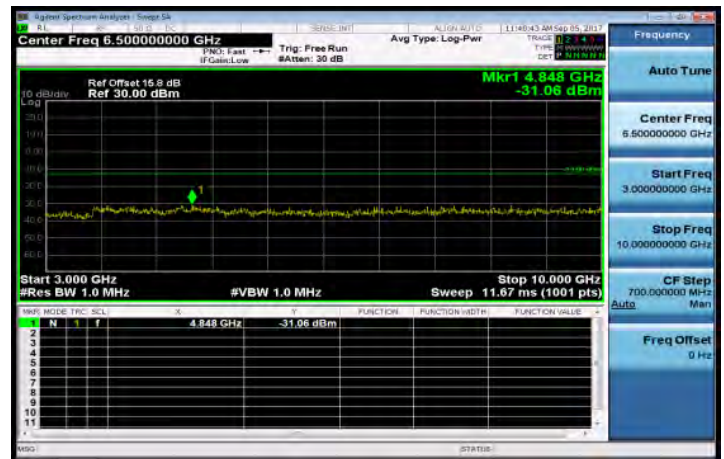
3GHz-10GHz_Band26_5MHz_QPSK_1_0_LowCH26715-816.5
