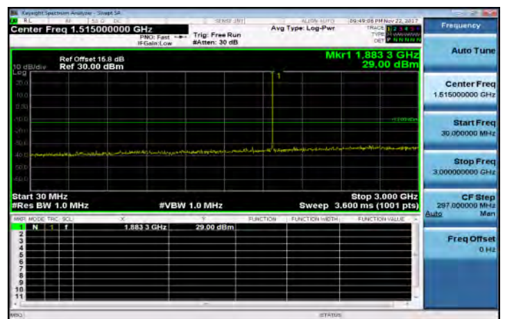
30MHz-3GHz_Band25_1_4MHz_QPSK_1_0_MidCH26365-1882.5
