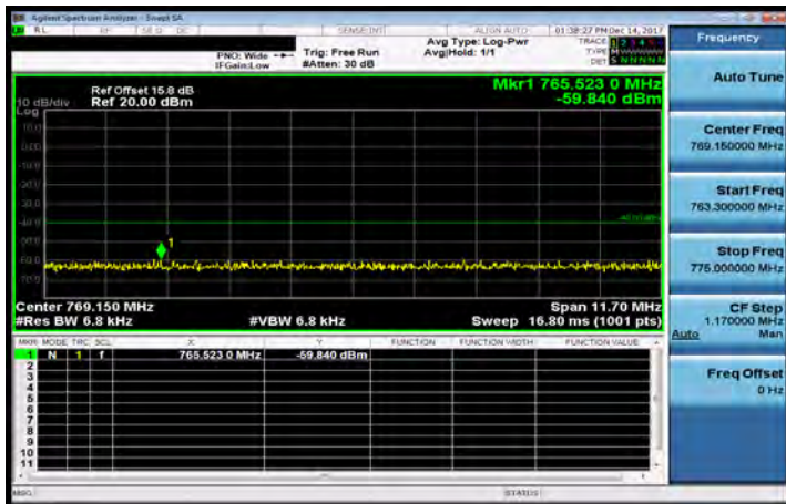
763.3MHz~775MHz_Band13_5MHz_QPSK_1_0_MidCH23230-782
