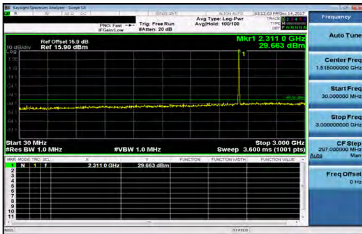
30MHz-3GHz_Band30_5MHz_QPSK_1_0_HighCH27735
