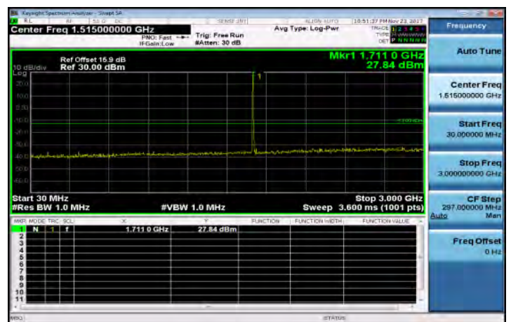
30MHz-3GHz_Band66_5MHz_QPSK_1_0_LowCH131997
