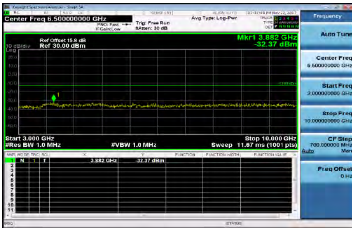
3GHz-10GHz_Band17_5MHz_QPSK_1_0_MidCH23790-710
