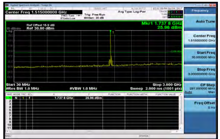
30MHz-3GHz_Band4_20MHz_QPSK_1_0_HighCH20300-1745
