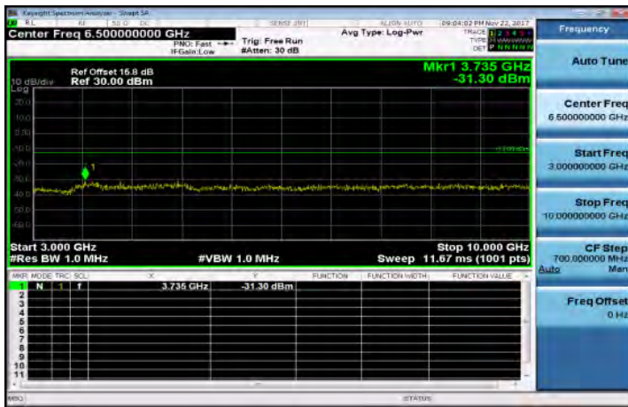
3GHz-10GHz_Band17_10MHz_QPSK_1_0_MidCH23790-710
