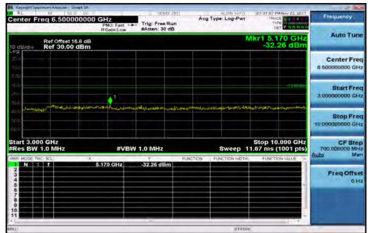
3GHz-10GHz_Band17_5MHz_QPSK_1_0_LowCH23755-706.5
