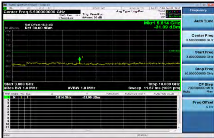
3GHz-10GHz_Band26_3MHz_OPSK_1_0_LowCH26705
