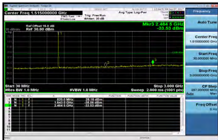
30MHz-3GHz_Band26_5MHz_OPSK_1_0_HighCH2675
