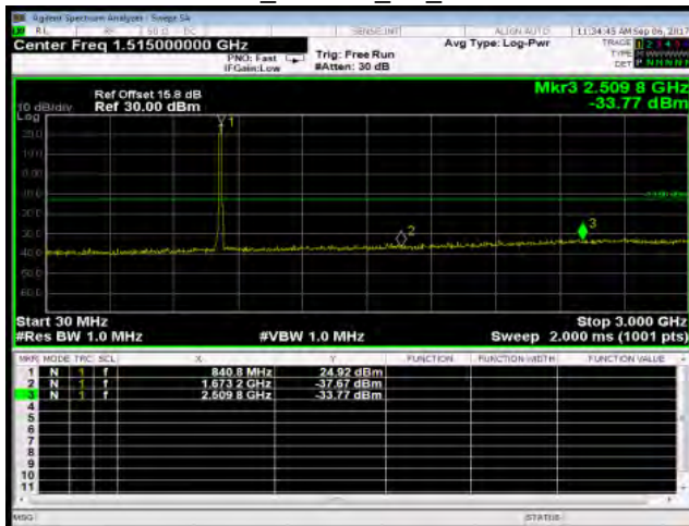
30MHz~3GHz_HSDPA_B5_MidCH4183-836.6
