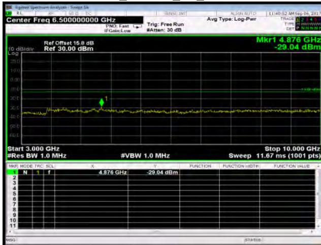
3GHz~10GHz_HSUPA_B5_LowCH4132-826.4
