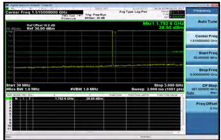
30MHz-3GHz_Band4_3MHz_QPSK_1_0_HighCH20385-1753.5
