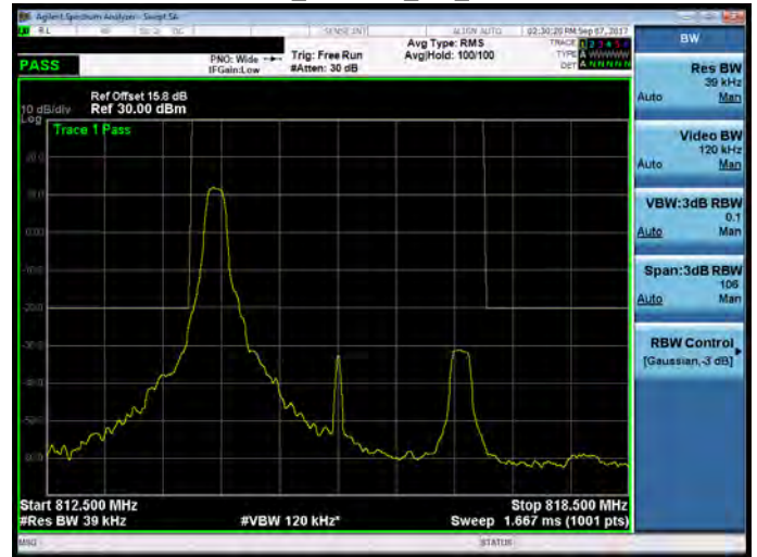
Part 90_Band 26_3M_1RB14
