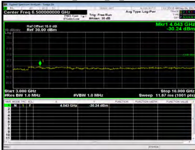
3GHz~10GHz_HSDPA_B5_LowCH4132-826.4
