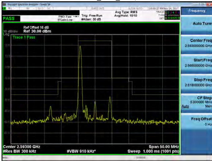
Band 41_10M_RB1,49
