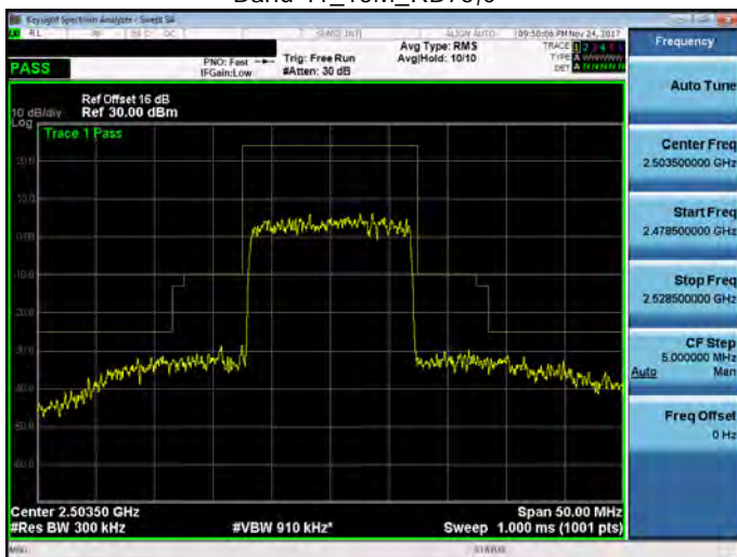
Band 41_15M_RB75,0
