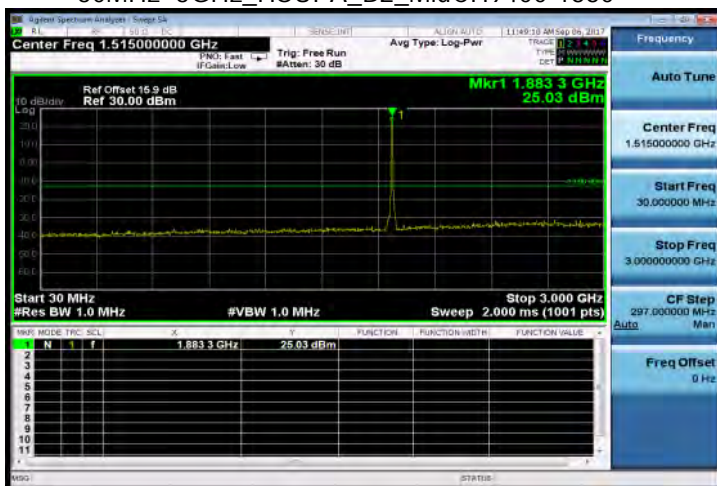
30MHz~3GHz_HSUPA_B2_MidCH9400-1880
