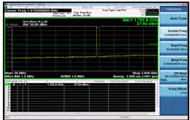
30MHz-3GHz_Band4_5MHz_QPSK_1_0_HighCH20375-1752.5
