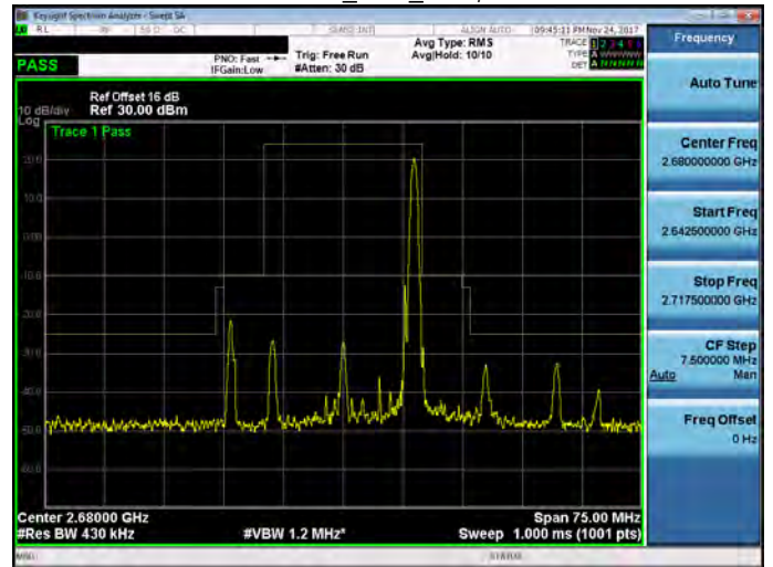
Band 41_20M_RB100,0
