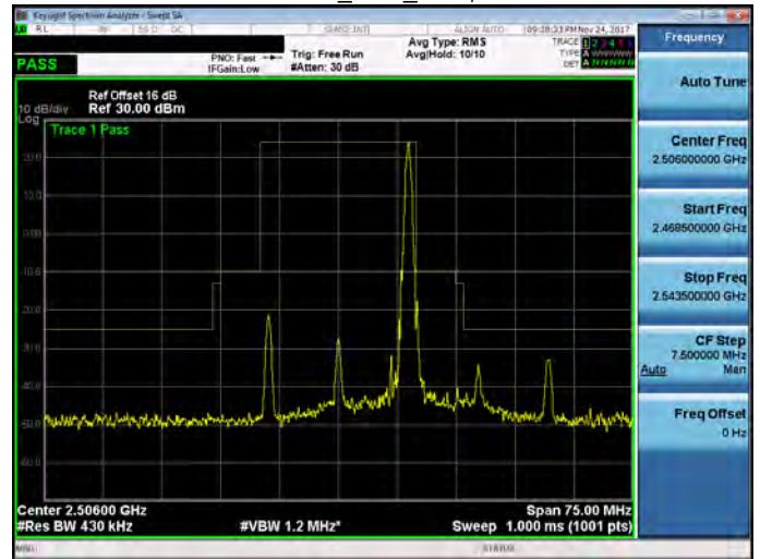
Band 41_20M_RB100,0
