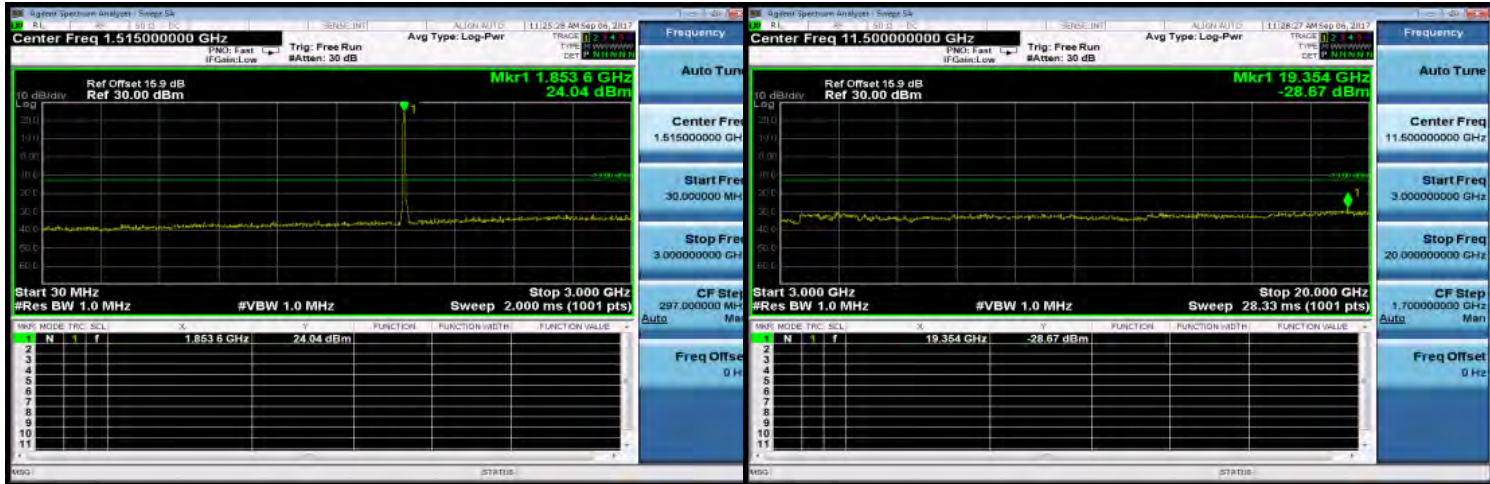
30MHz-3GHz_HSDPA_B2_LowCH9262-1852.4
