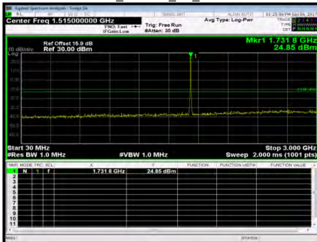
30MHz~3GHz_HSUPA_B4_MidCH1413-1732.6
