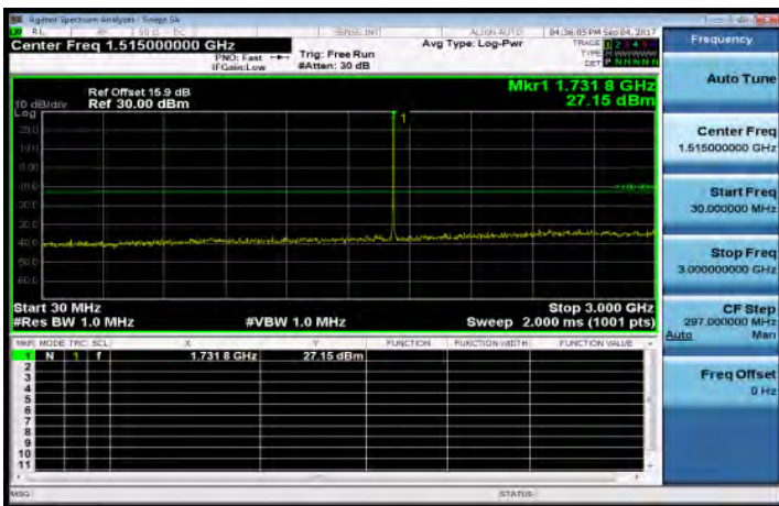
30MHz-3GHz_Band4_3MHz_QPSK_1_0_MidCH20175-1732.5
