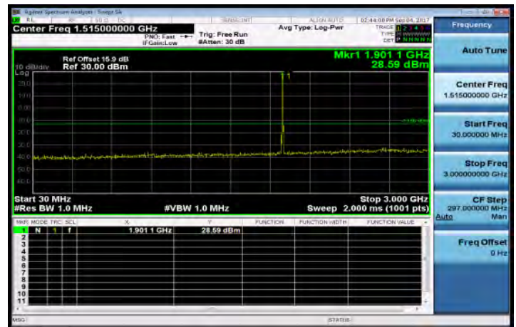
30MHz-3GHz_Band2_10MHz_QPSK_1_0_HighCH19150-1905
