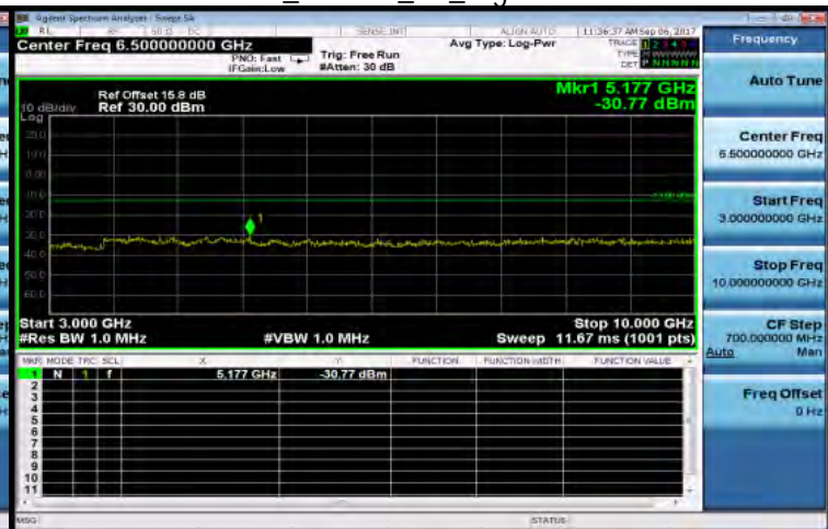
3GHz~10GHz_HSDPA_B5_HighCH4233-846.6
