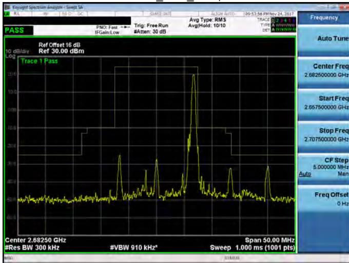
Band 41_15M_RB75,0
