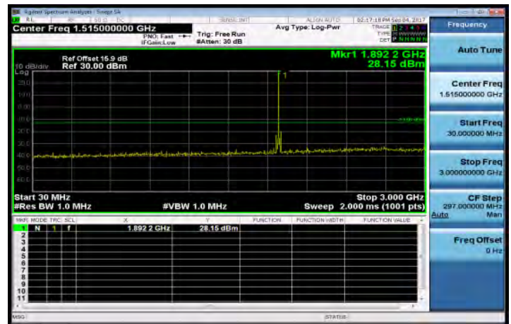
30MHz-3GHz_Band2_20MHz_QPSK_1_0_HighCH19100-1900
