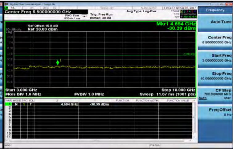
3GHz~10GHz_HSUPA_B5_MidCH4183-836.6
