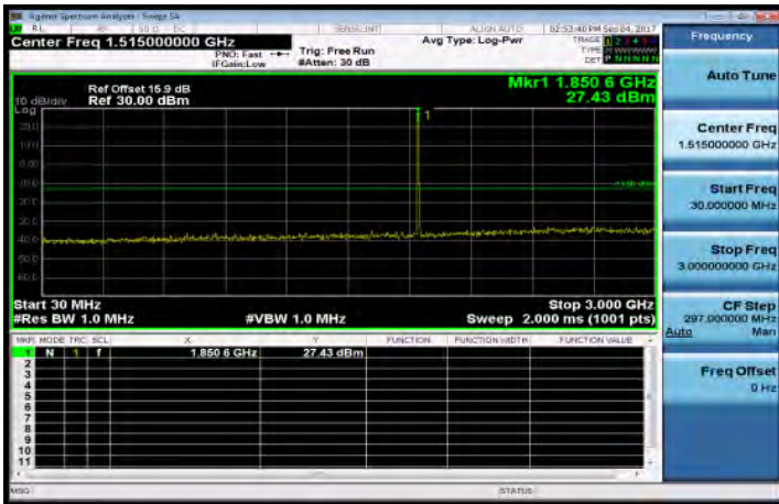
30MHz-3GHz_Band2_5MHz_QPSK_1_0_LowCH18625-1852.5
