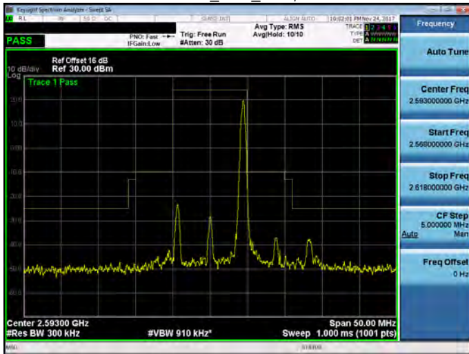
Band 41_10M_RB50,0
