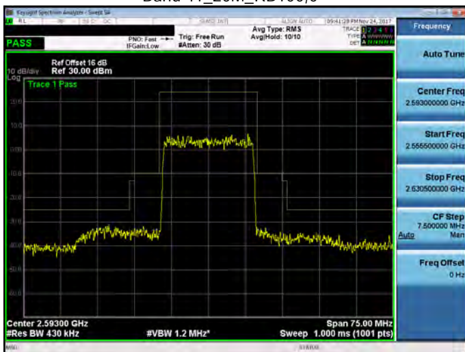
Band 41_20M_RB100,0
