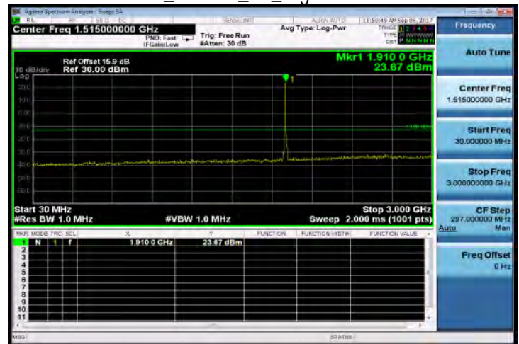
30MHz~3GHz_HSUPA_B2_HighCH9538-1907.6
