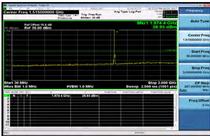
30MHz-3GHz_Band2_15MHz_QPSK_1_0_MidCH18900-1880
