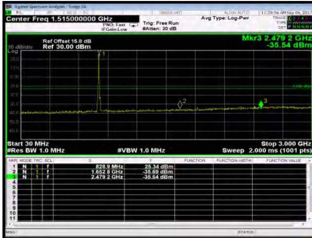
30MHz~3GHz_HSUPA_B5_LowCH4132-826.4
