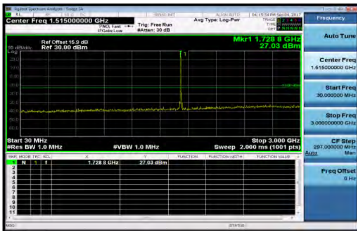
30MHz-3GHz_Band4_10MHz_QPSK_1_0_MidCH20175-1732.5
