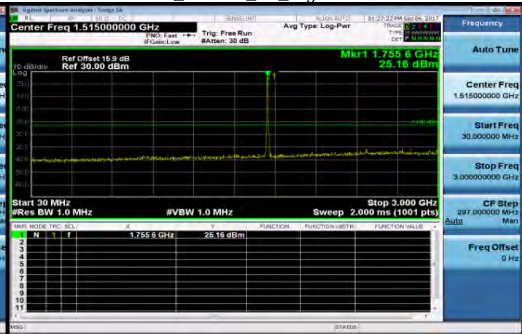
30MHz~3GHz_HSUPA_B4_HighCH1513-1752.6
