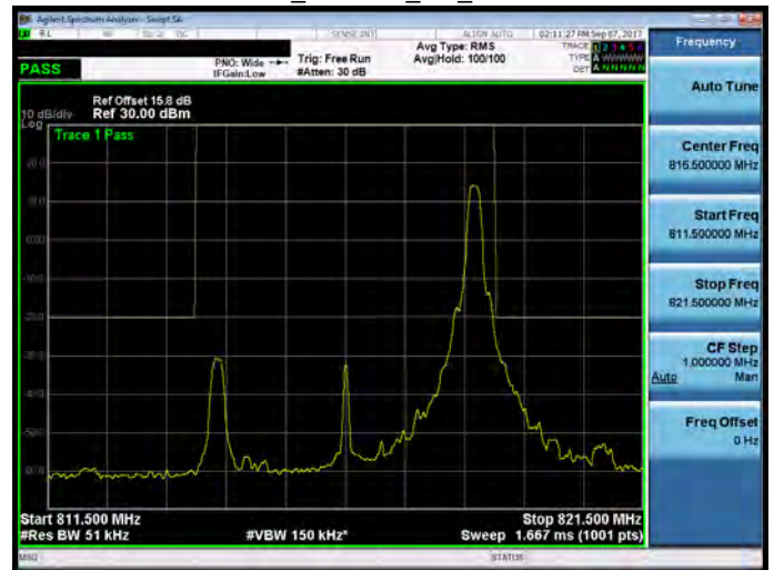
Part 90_Band 26_5M_25RB0
