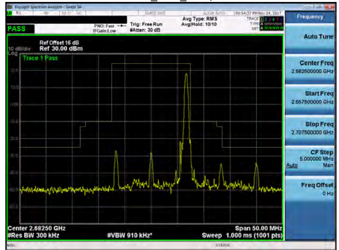
Band 41_15M_RB75,0
