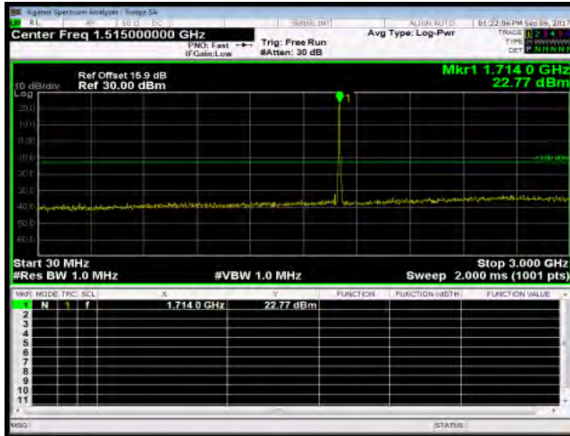
30MHz~3GHz_HSUPA_B4_LowCH1312-1712.4
