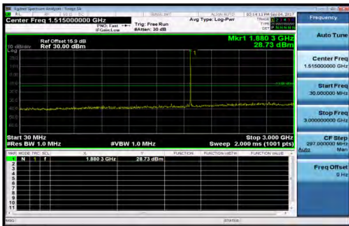
30MHz-3GHz_Band2_3MHz_QPSK_1_0_MidCH18900-1880
