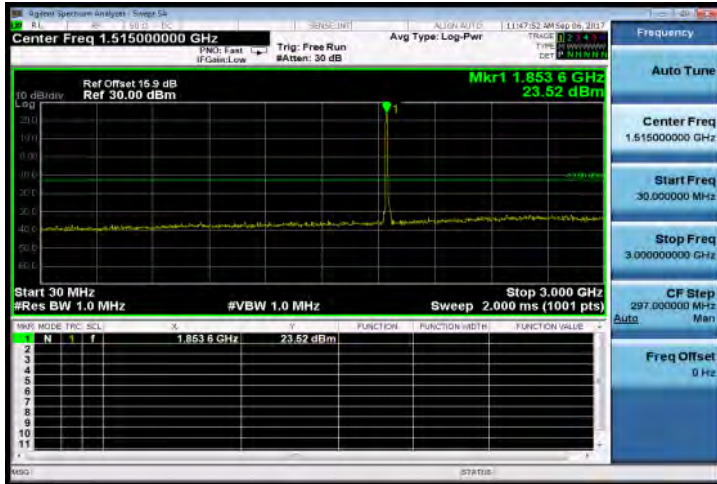
30MHz~3GHz_HSUPA_B2_LowCH9262-1852.4
