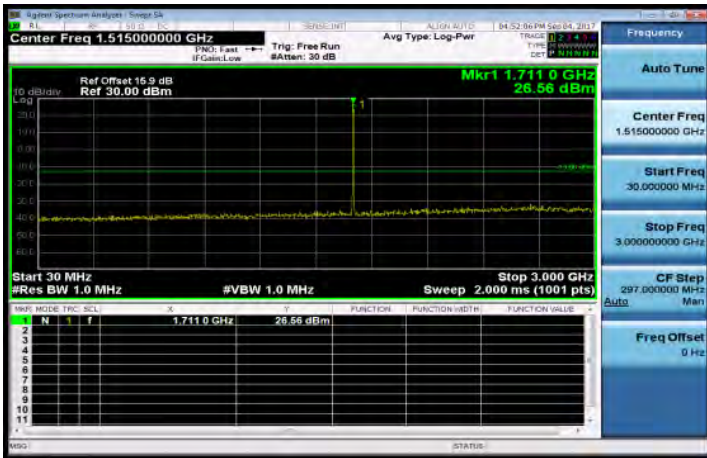
30MHz-3GHz_Band4_1_4MHz_QPSK_1_0_LowCH19957-1710.7
