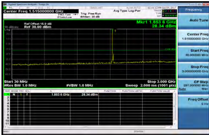
30MHz-3GHz_Band2_20MHz_QPSK_1_0_LowCH18700-1860
