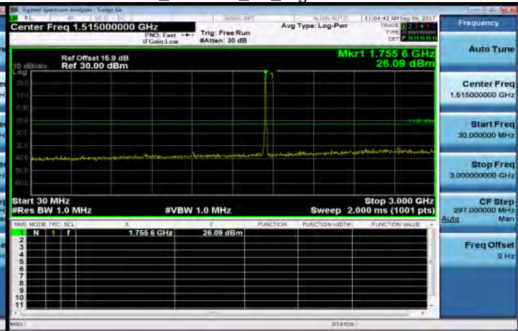
30MHz~3GHz_WCDMA_B4_HighCH1513-1752.6
