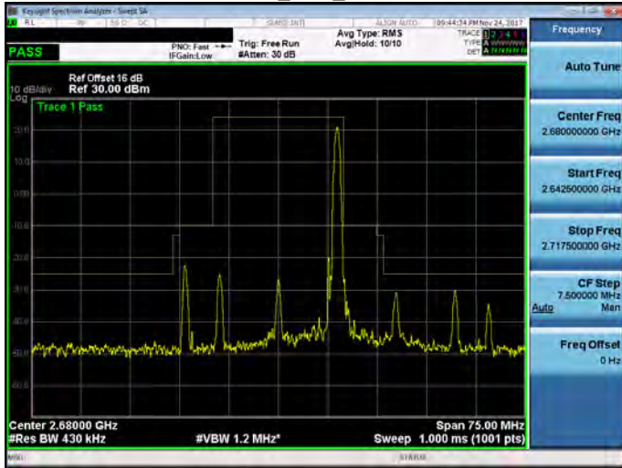
Band 41_20M_RB100,0
