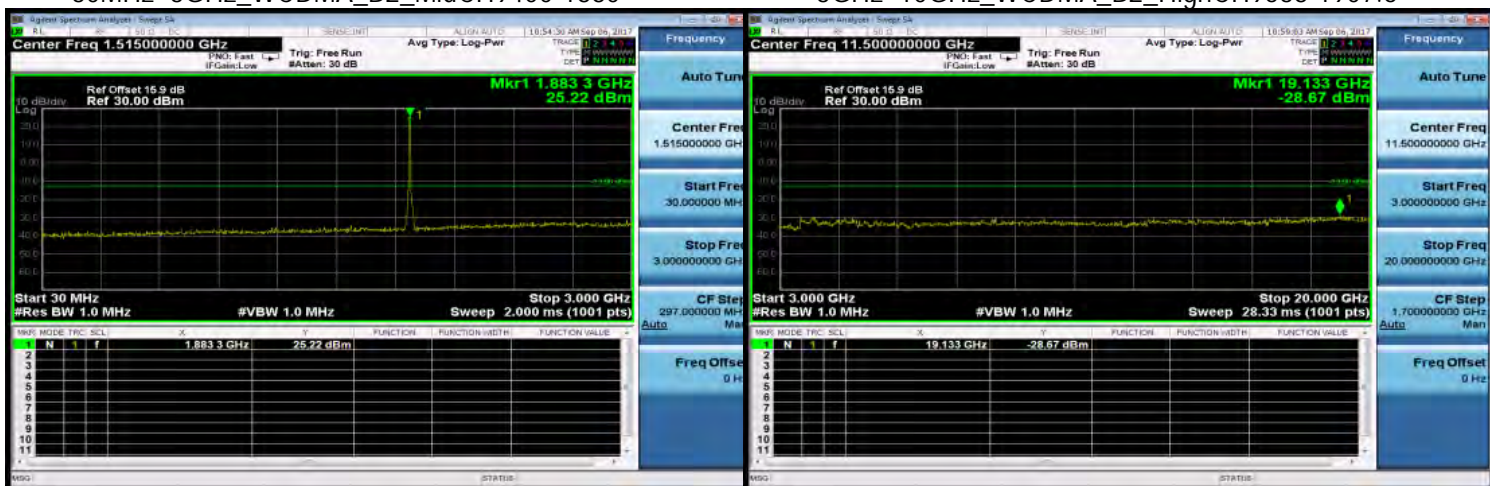
30MHz~3GHz_WCDMA_B2_MidCH9400-1880
