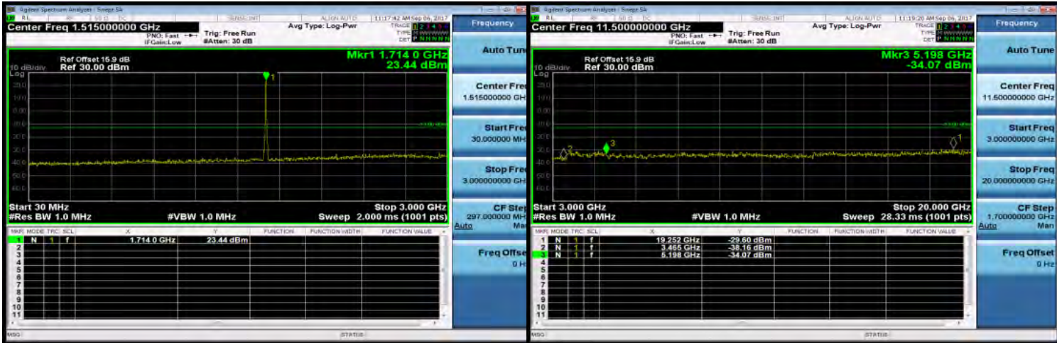
30MHz~3GHz_HSDPA_B4_LowCH1312-1712.4
