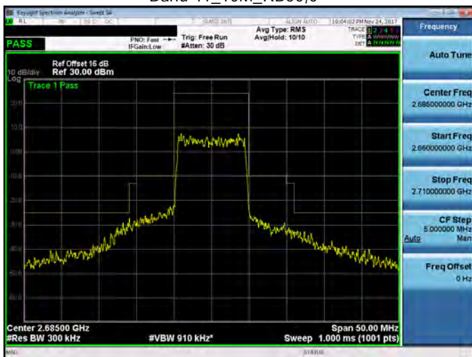
Band 41_10M_RB50,0
