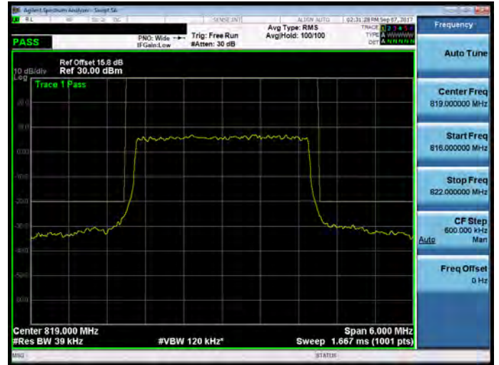
Part 90_Band 26_3M_1RB0
