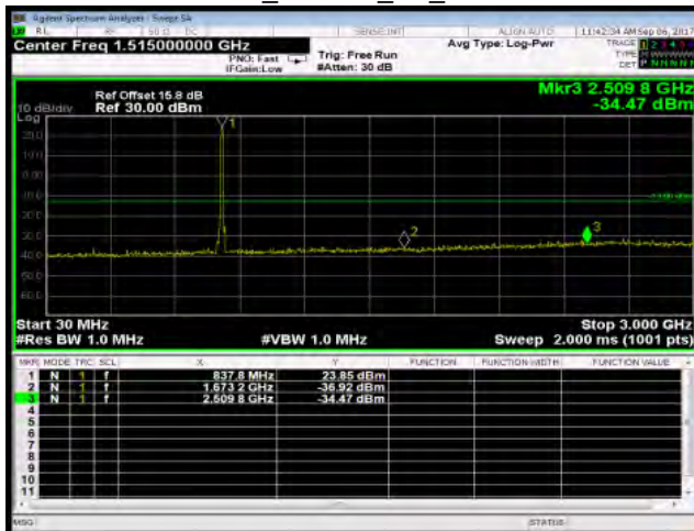
30MHz~3GHz_HSUPA_B5_MidCH4183-836.6
