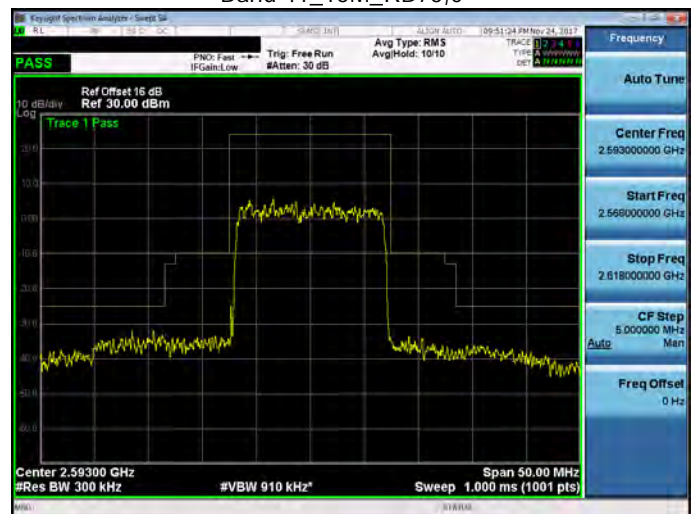
Band 41_15M_RB75,0
