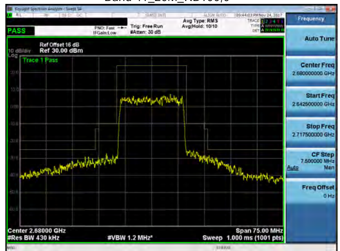
Band 41_20M_RB100,0
