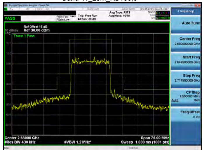
Band 41_20M_RB100,0
