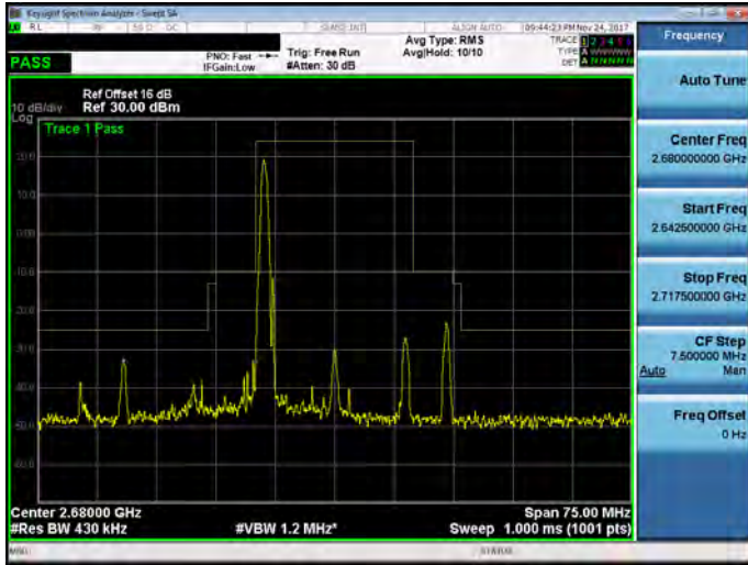
Band 41_20M_RB1,99
