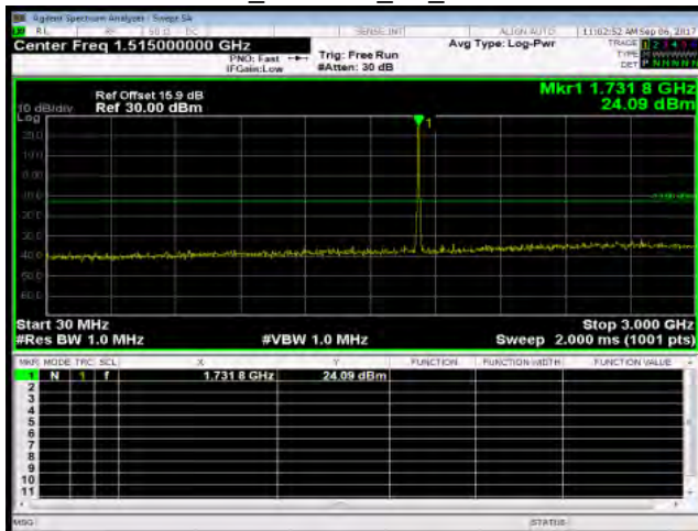
30MHz~3GHz_WCDMA_B4_MidCH1413-1732.6
