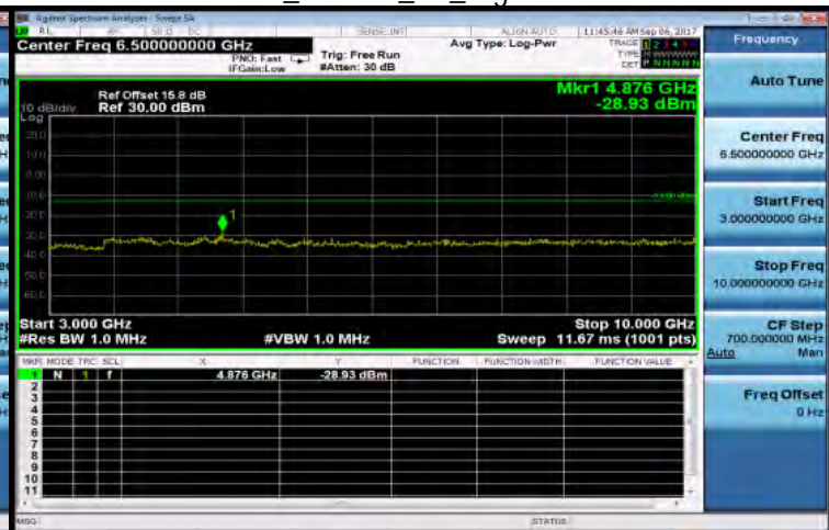
3GHz~10GHz_HSUPA_B5_HighCH4233-846.6
