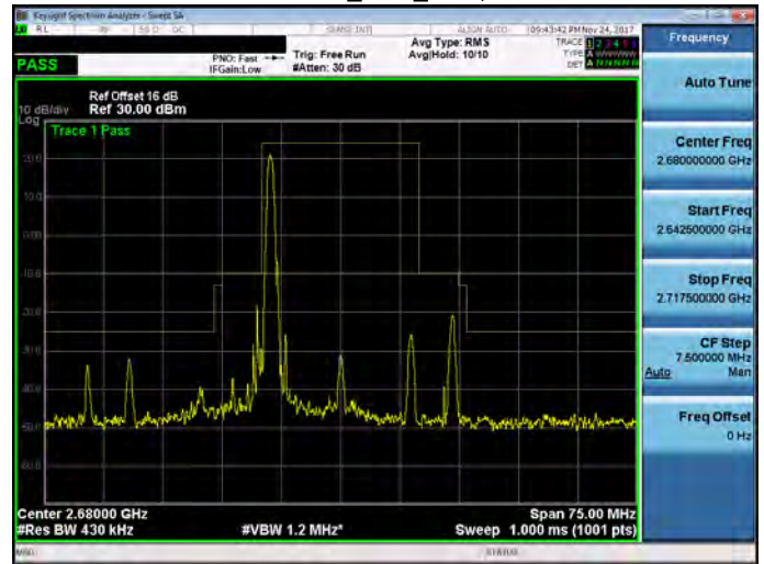
Band 41_20M_RB1,99
