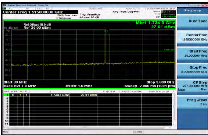
30MHz-3GHz_Band4_1_4MHz_QPSK_1_0_MidCH20175-1732.5
