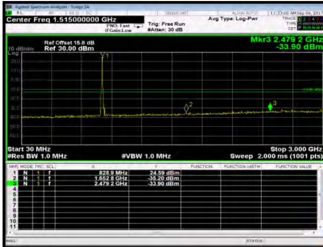
30MHz~3GHz_HSDPA_B5_LowCH4132-826.4
