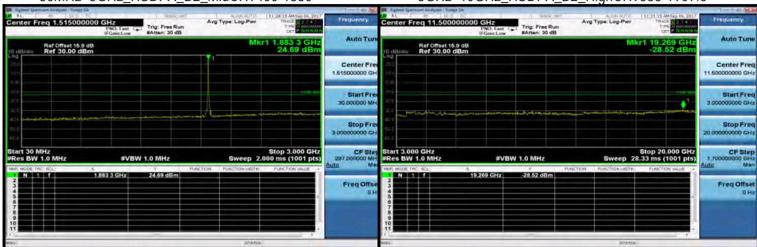
30MHz-3GHz_HSDPA_B2_MidCH9400-1880
