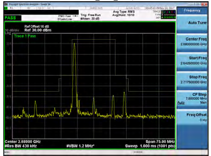
Band 41_20M_RB1,99
