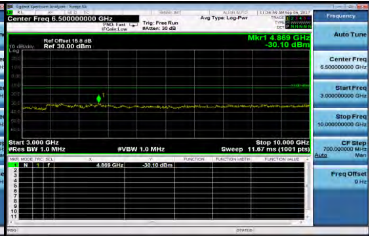
3GHz~10GHz_HSDPA_B5_MidCH4183-836.6
