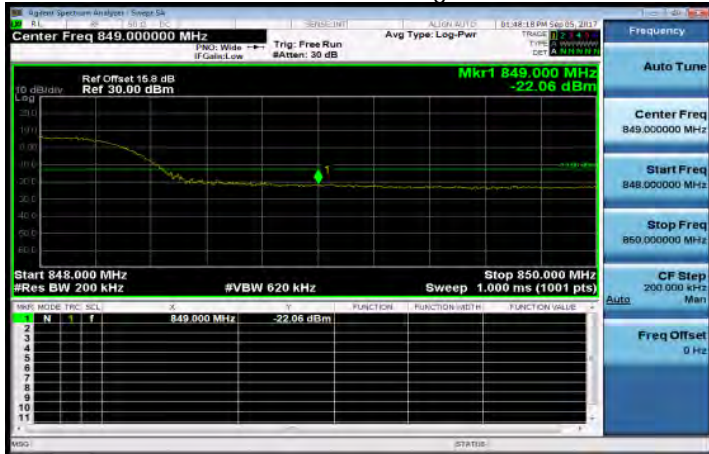
Band26_15MHz_QPSK_75_0_HighCH26965-841.5
