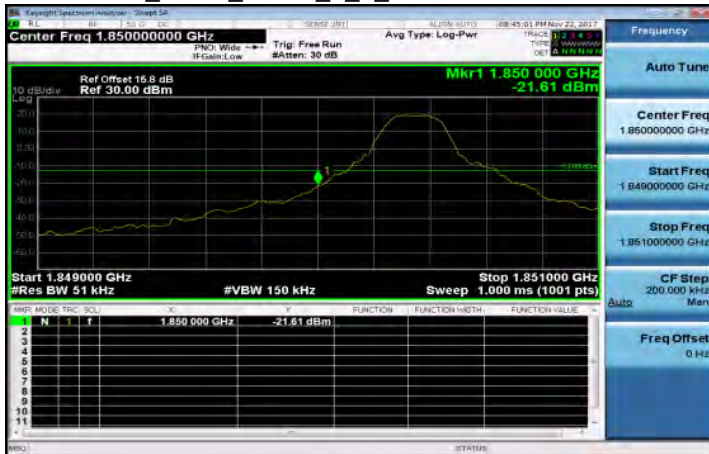
Band25_5MHz_QPSK_1_0_LowCH26065-1852.5
