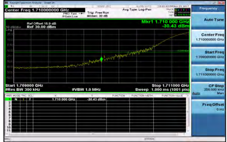
Band66_20MHz_QPSK_1_0_LowCH132072
