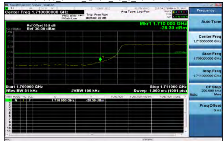
Band66_5MHz_QPSK_25_0_LowCH131997
