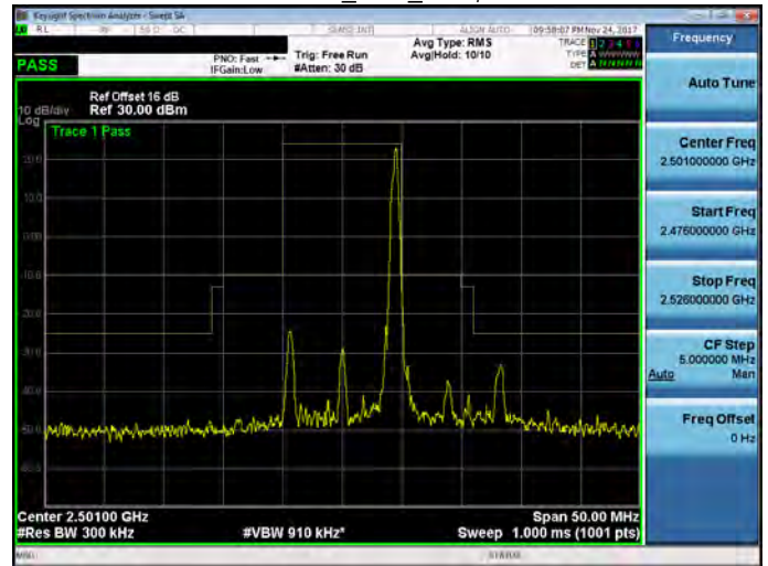
Band 41_10M_RB50,0
