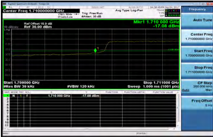
Band4_3MHz_QPSK_15_0_LowCH19965-1711.5
