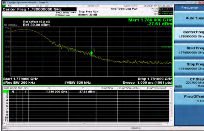
Band66_15MHz_QPSK_1_74_HighCH132597
