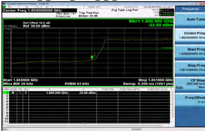
Band25_1_4MHz_QPSK_6_0_LowCH26047-1850.7
