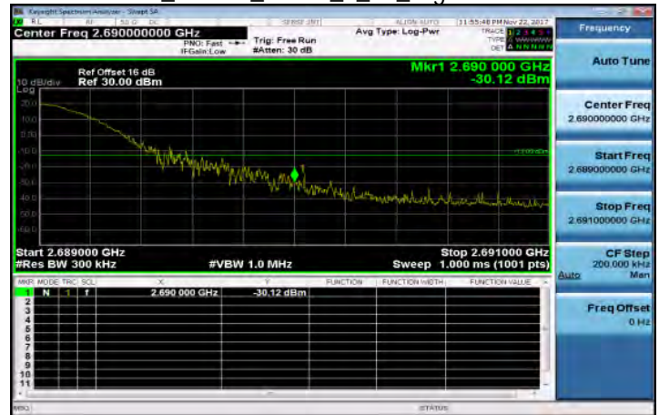
Band41_20MHz_QPSK_1_99_HighCH41490
