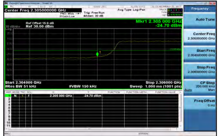
Band30_5MHz_QPSK_25_0_LowCH27685
