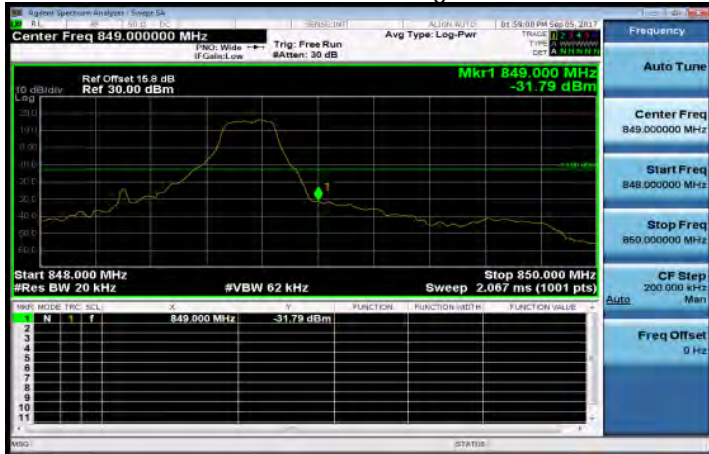
Band26_1_4MHz_QPSK_1_5_HighCH27033-848.3
