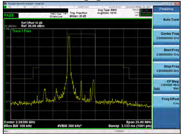
Band 41_5M_RB1,24
