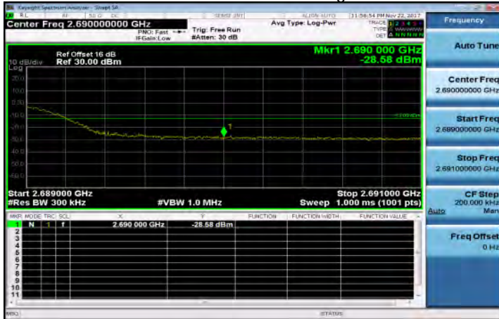
Band41_20MHz_QPSK_100_0_HighCH41490
