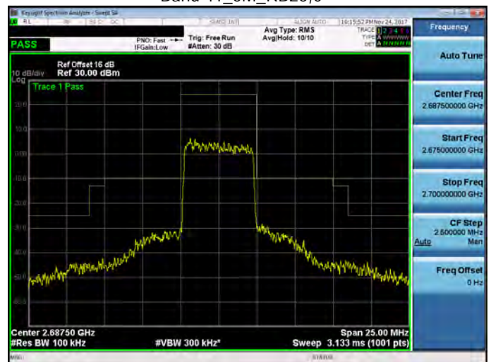
Band 41_5M_RB25,0
