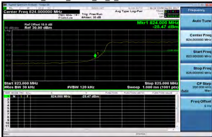
Band5_3MHz_QPSK_15_0_LowCH20415-825.5
