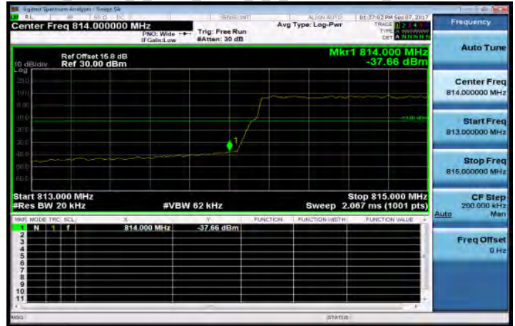
Part 90_Band26_1_4MHz_QPSK_6_0_LowCH26697_LowCH26697
