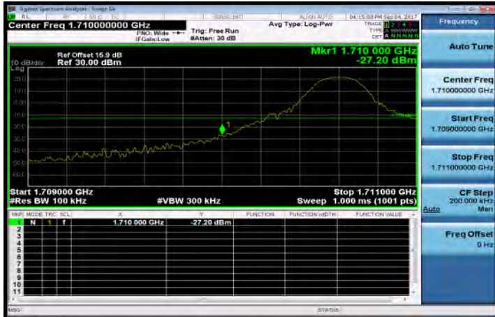
Band4_10MHz_QPSK_1_0_LowCH20000-1715
