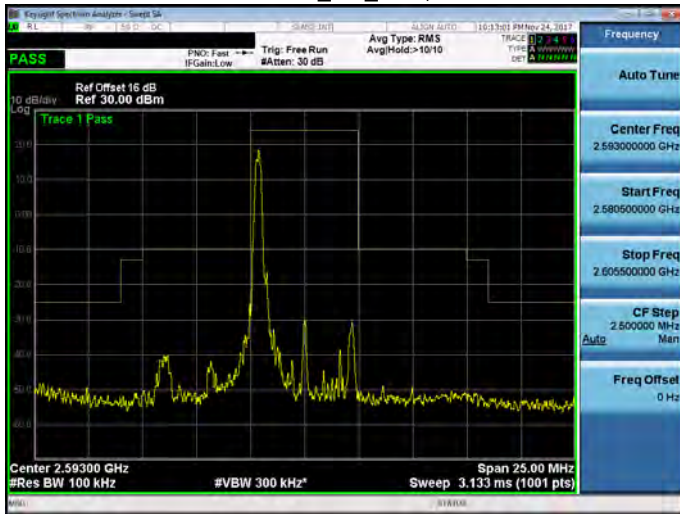
Band 41_5M_RB1,24
