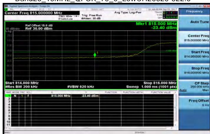
Band26_15MHz_QPSK_75_0_LowCH26825-822.5
