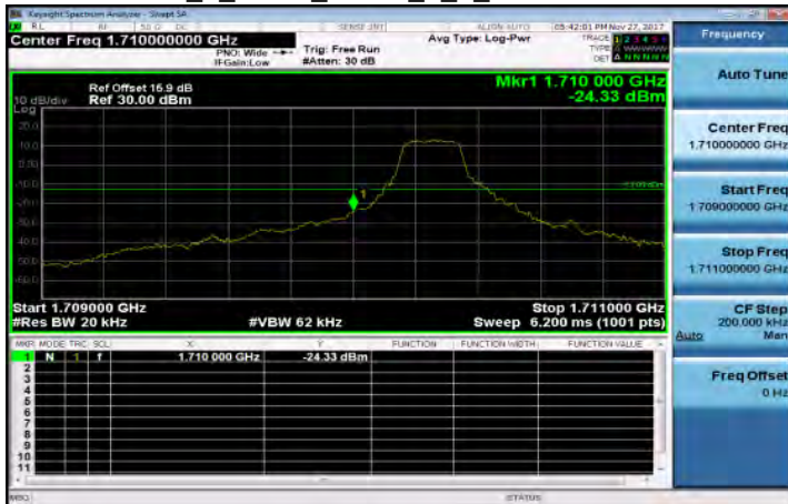
Band66_1_4MHz_QPSK_1_0_LowCH131979
