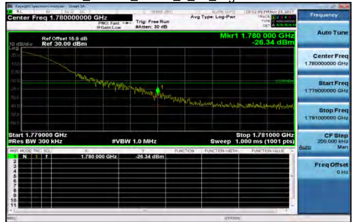
Band66_20MHz_QPSK_1_99_HighCH132572
