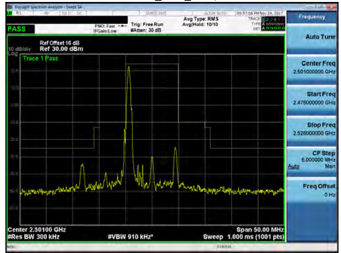
Band 41_10M_RB1,49
