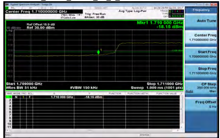
Band4_5MHz_QPSK_25_0_LowCH19975-1712.5
