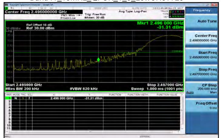
Band41_15MHz_QPSK_1_0_LowCH39725
