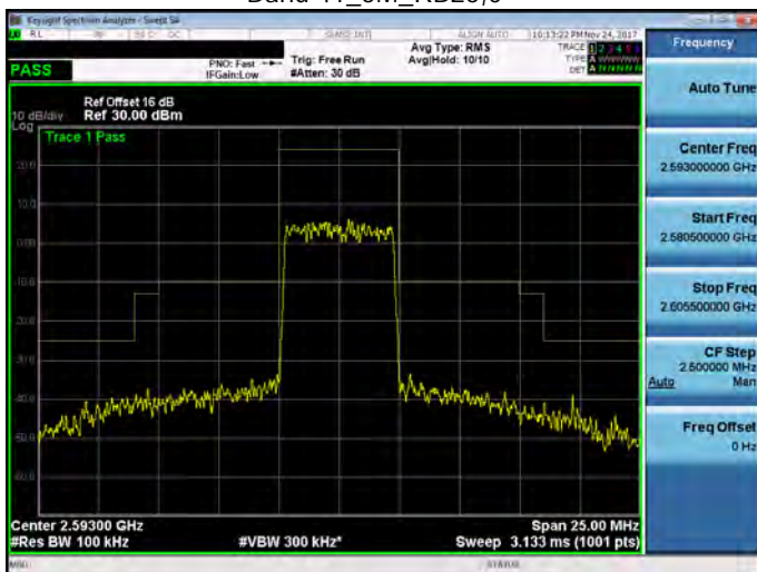
Band 41_5M_RB25,0
