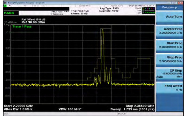
Emission Mask Band 30_10M_RB1,0_ch_27710
