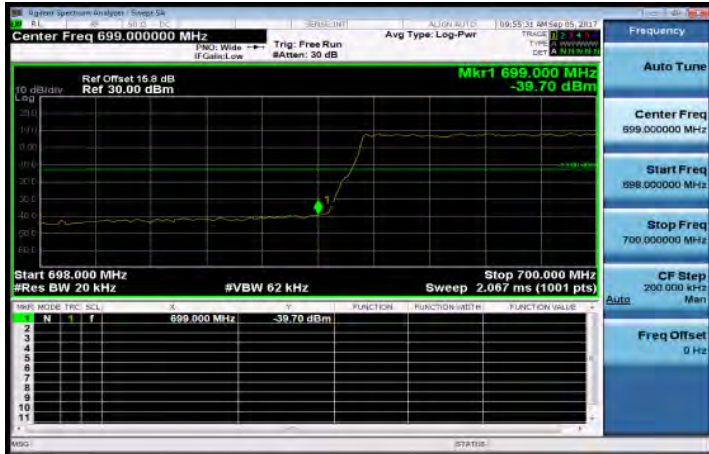
Band12_1_4MHz_QPSK_6_0_LowCH23017-699.7
