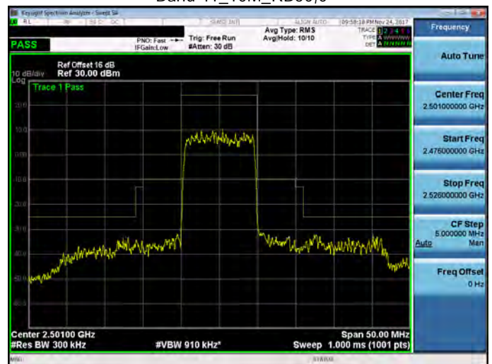
Band 41_10M_RB50,0
