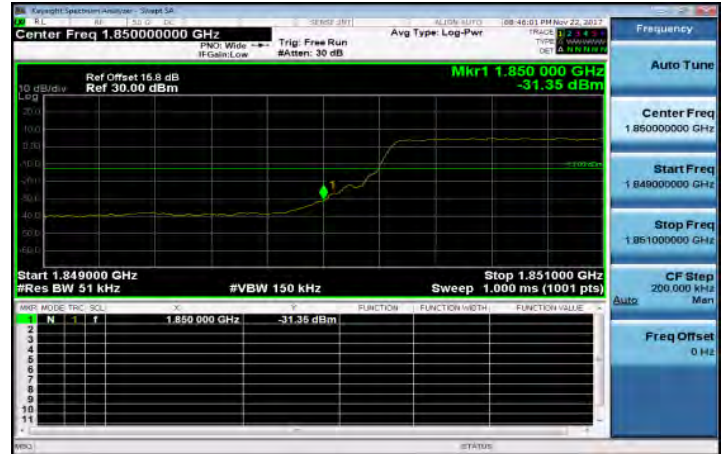
Band25_5MHz_QPSK_25_0_LowCH26065-1852.5
