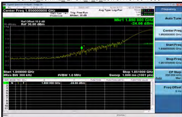
Band2_20MHz_QPSK_1_0_LowCH18700-1860
