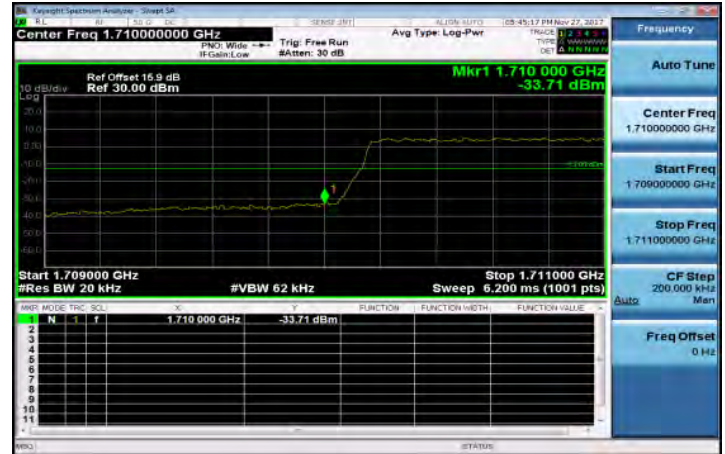
Band66_1_4MHz_QPSK_6_0_LowCH131979
