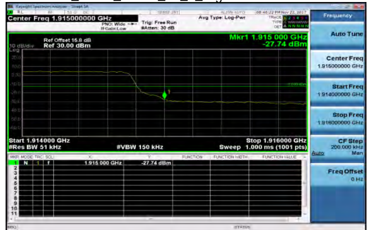
Band25_5MHz_QPSK_25_0_HighCH26665-1912.5
