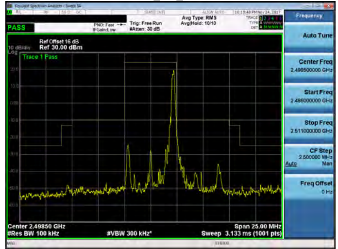
Band 41_5M_RB25,0
