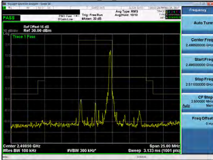
Band 41_5M_RB25,0
