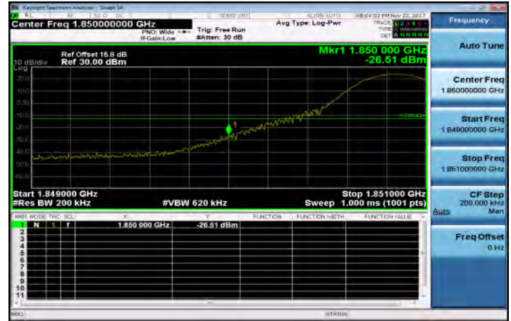
Band25_15MHz_QPSK_1_0_LowCH26115-1857.5
