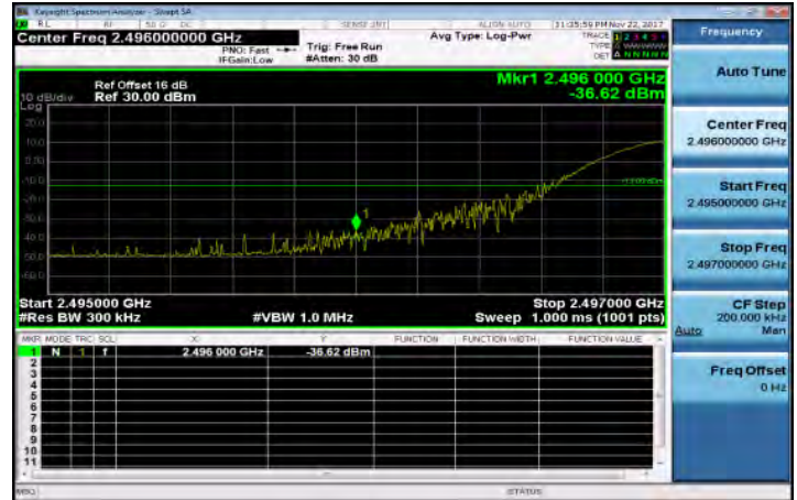
Band41_20MHz_QPSK_1_0_LowCH39750
