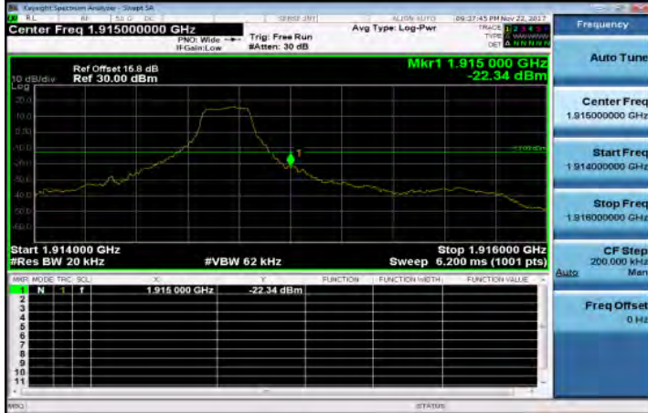
Band25_1_4MHz_QPSK_1_5_HighCH26683-1914.3
