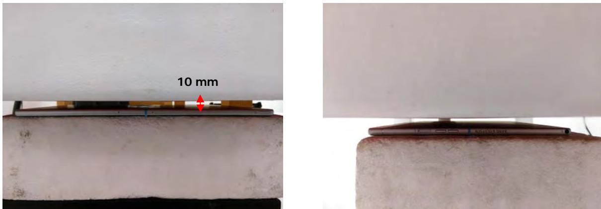
Fig.4 EUT Back side (10mm) to flat phantom
