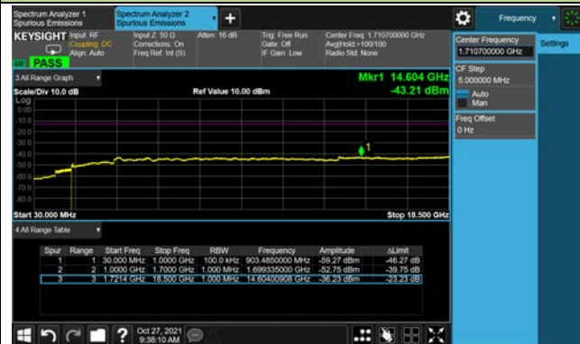
Channel 132665 (1779.3MHz)
