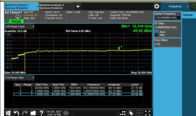
Channel 26683 (1914.3MHz)
