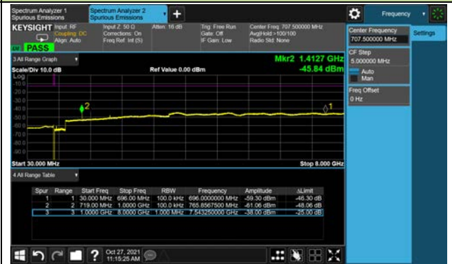
Channel 23095 (707.5MHz)
