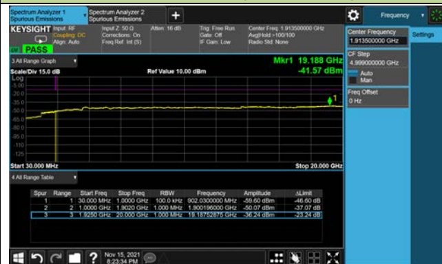
Channel 26675 (1913.5MHz)
