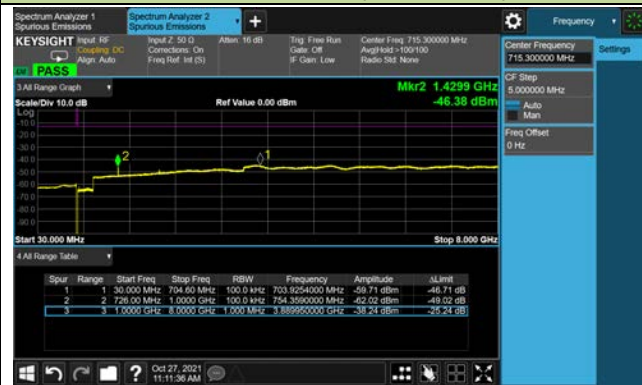
Channel 23173 (715.3MHz)
