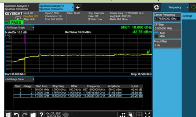
Channel 132657 (1778.5MHz)
