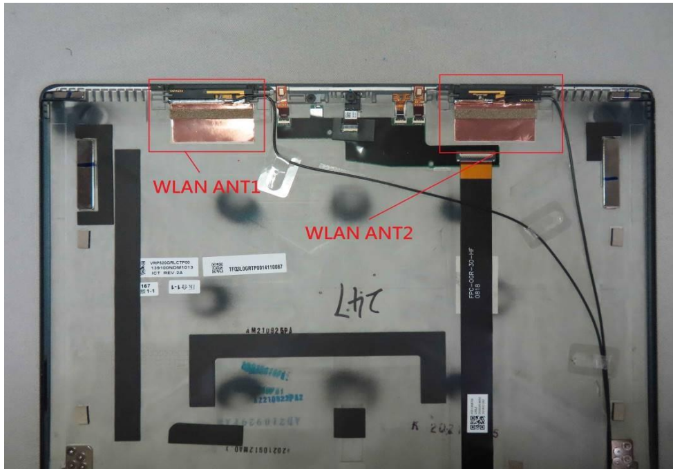
WLAN Antenna
