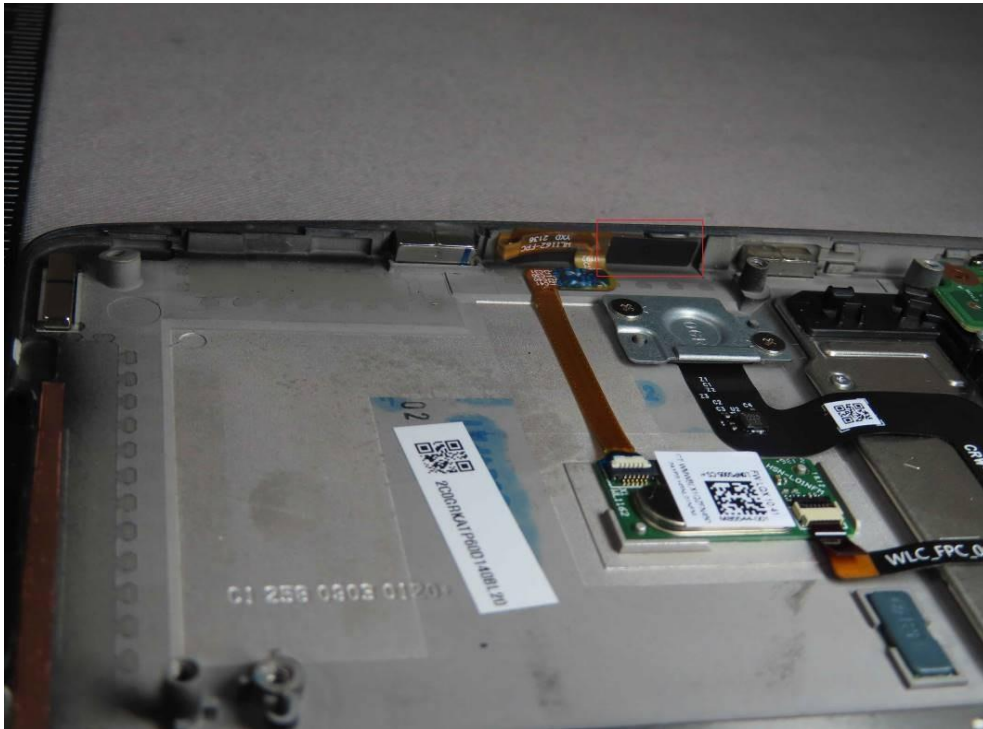
WLAN Antenna
