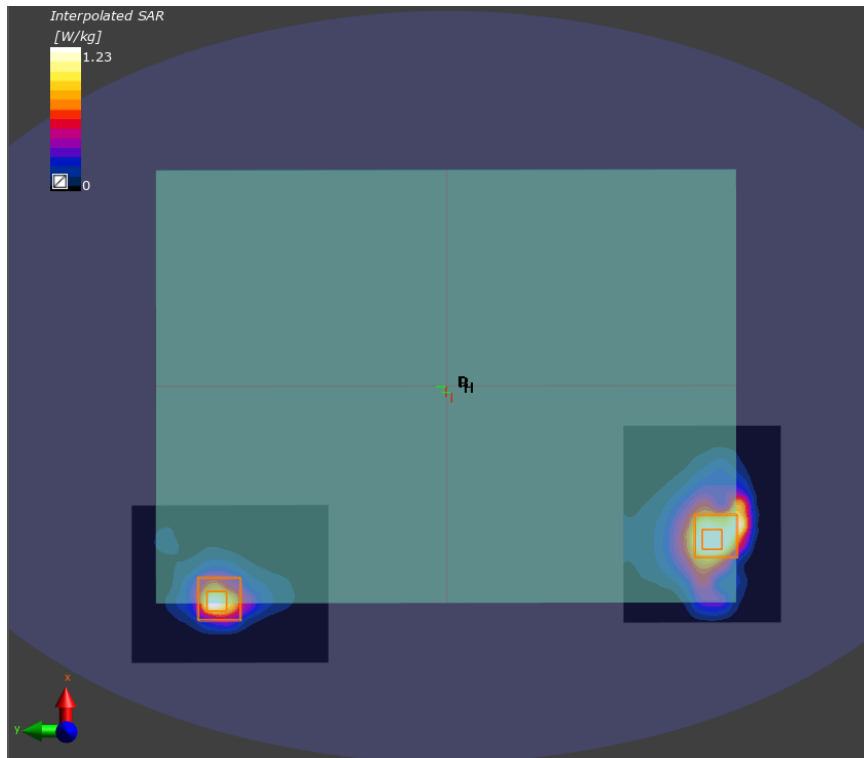
WLAN/BT Main and Aux hotspot location
