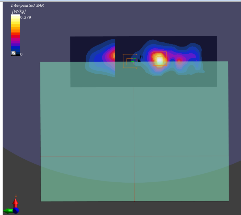
WLAN/BT Main and Aux hotspot location
