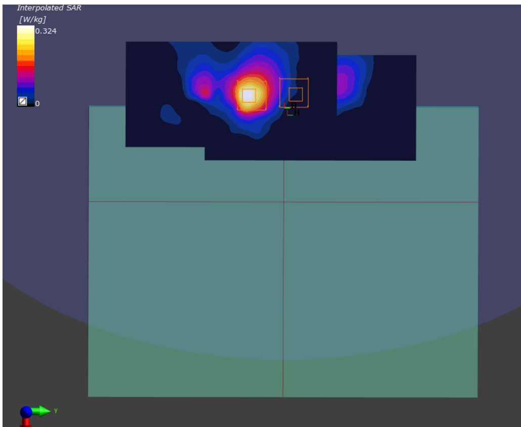
WLAN/BT Main and Aux hotspot location
